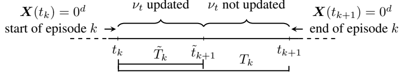
Figure 1: MDP evolution in episode k < K_T .
