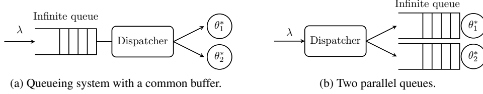
Figure 2: Two-server queueing systems with heterogeneous service rates.
