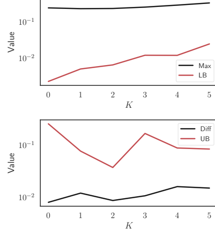
Figure 3. Results for synthetic experiments on real-world data. \text{Diff} := Err_{\mathcal{D}(h_S^*)}(h_S^*) - Err_{\mathcal{D}(h_T^*)}(h_T^*) , \text{Max} := \max\{Err_{\mathcal{D}_S}(h_S^*), Err_{\mathcal{D}(h_T^*)}(h_T^*)\} , \text{UB} := upper bound specified in Theorem 4.2, and \text{LB} := lower bound specified in Theorem 4.6. For each time step K = k , we compute and deploy the source optimal classifier h_S^* and update the credit score for each individual according to the received decision as the new reality for time step K = k + 1 . Details of the data generation are deferred to Appendix D.
