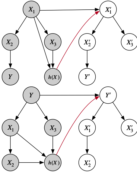
Figure 2. Example causal graph annotated to demonstrate covariate shift (Up) / target shift (Down) as a result of the deployment of h . Grey nodes indicate observable variables and transparent nodes are not observed at the training stage. Red arrow emphasizes h induces changes in certain variables.
