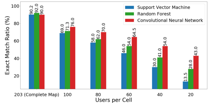
Fig. 15. Performance comparison of ML models on scarce and complete coverage maps data [140].
