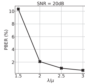
(b) \lambda/\mu v.s. PBER
