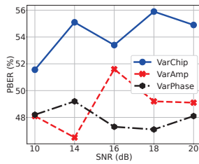
Figure 11: No POTP.
