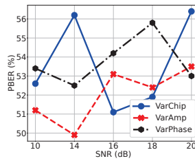
Figure 12: Fake POTPs.
