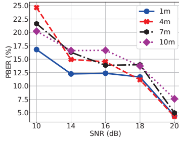
(b) VarChip at Hallway
