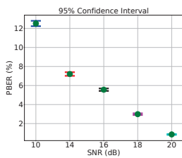
(o) VarPhase at Hallway (1 m)
