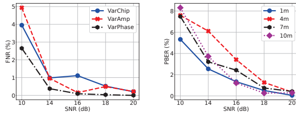
Figure 14: FNR performance. Figure 15: PBER ( r = 3 ).
