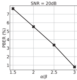
(a) \alpha/\beta v.s. PBER
