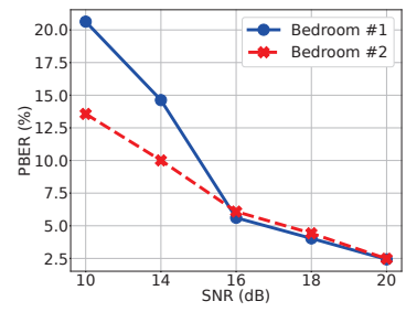
(f) VarAmp at Apartment
