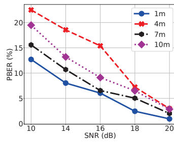
(e) VarAmp at Hallway
