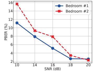
(i) VarPhase at Apartment
