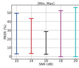
(c) VarAmp at Lab (7 m)
