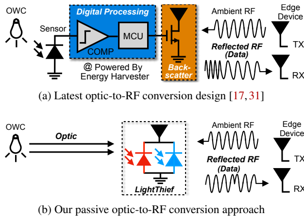
Figure 2: Comparison between different optic-to-RF conversion approaches.
