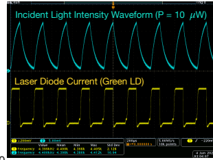
Figure 9: LD current waveform vs. light intensity waveform
