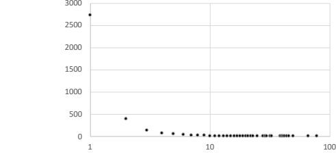
Fig. 4: Degree of constructor polymorphism. The X-axis/Y-axis denotes the number of distinct object types/classes.
