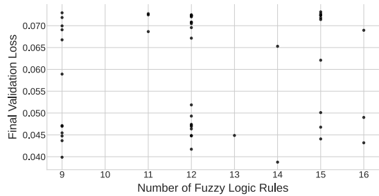
Fig. 6. Plotting each trial as a marker, the Latent Lockstep Method was used on 32 continuous input data to show the relationship between the number of fuzzy logic rules and the FLC’s final validation loss (lower is better).
