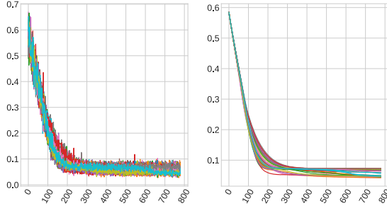
Fig. 1. The Latent Lockstep Method: (left) training loss; (right) validation loss. The x -axis is the batches.
