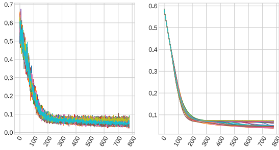
Fig. 5. The Latent Lockstep Method: (left) training loss; (right) validation loss. The x -axis is the batches.
