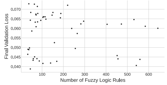
Fig. 4. Plotting each trial as a marker, the WM-EC Method was used on 8 continuous input data to show the relationship between the number of fuzzy logic rules and the FLC's final validation loss (lower is better).
