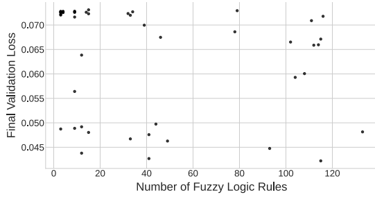
Fig. 2. Using the Latent Lockstep Method on 8 continuous input data, each trial is represented by a marker to display the relationship between the number of fuzzy logic rules and the FLC's final validation loss (lower is better).
