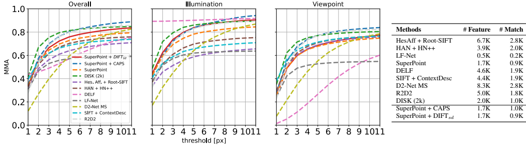
Figure 10: Mean Matching Accuracy (MMA) on HPatches [4]. For each method, we show the MMA with varying pixel error thresholds. We also report the mean number of detected features and mutual nearest neighbor matches. Although not trained with any explicit geometric correspondence labels, DIFT sd is able to achieve competitive performance compared to other feature descriptors that are specifically design or trained for this task.
