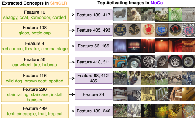
Figure 7. Transferring concepts from an explained representation space to an unseen representation space: We show that representations of self-supervised models can be mapped from one to another by learning a transformation \mathbf{Z} (See Equation 3). We transfer extracted concepts from SimCLR (source) (Chen et al., 2020a), to an unseen model, MoCo (target) (Chen et al., 2020b) by mapping the source features to the target features with the highest weights in \mathbf{Z} . We observe that the top activating images of the mapped features in the MoCo very closely match the concepts extracted in SimCLR.
