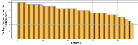
Figure A.6. Average agreement between participants for each feature: We plot the agreement of relevancy for each concept averaged by the feature for 93 features we perform human study on.
