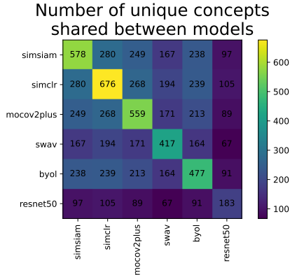
Figure A.1. Shared concepts between models: Among the unique concepts extracted using FALCON on the representation space of various models, we plot the number shared concepts between each pair of models.
