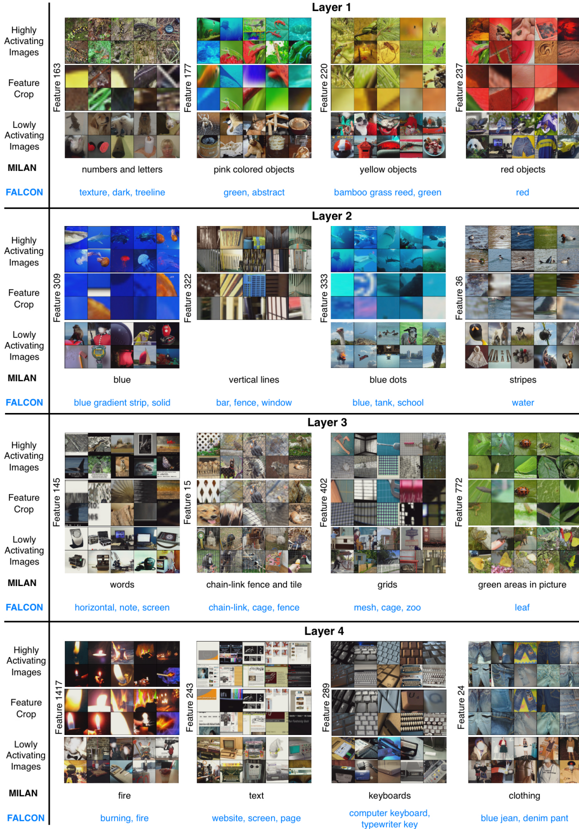
Figure A.8. Concepts for features of various layers of supervised ResNet-50: We extract concepts from random features of layers of supervised pre-trained ResNet-50. We compare FALCON concepts with MILAN concepts.
