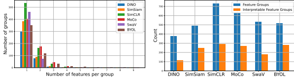
Figure A.2. Distribution of feature groups: For different self-supervised model representation spaces we compute the feature groups (from Algorithm 1). On the left we plot group sizes against the number of groups and on the right, we plot the number of interpretable groups among the discovered feature groups.
