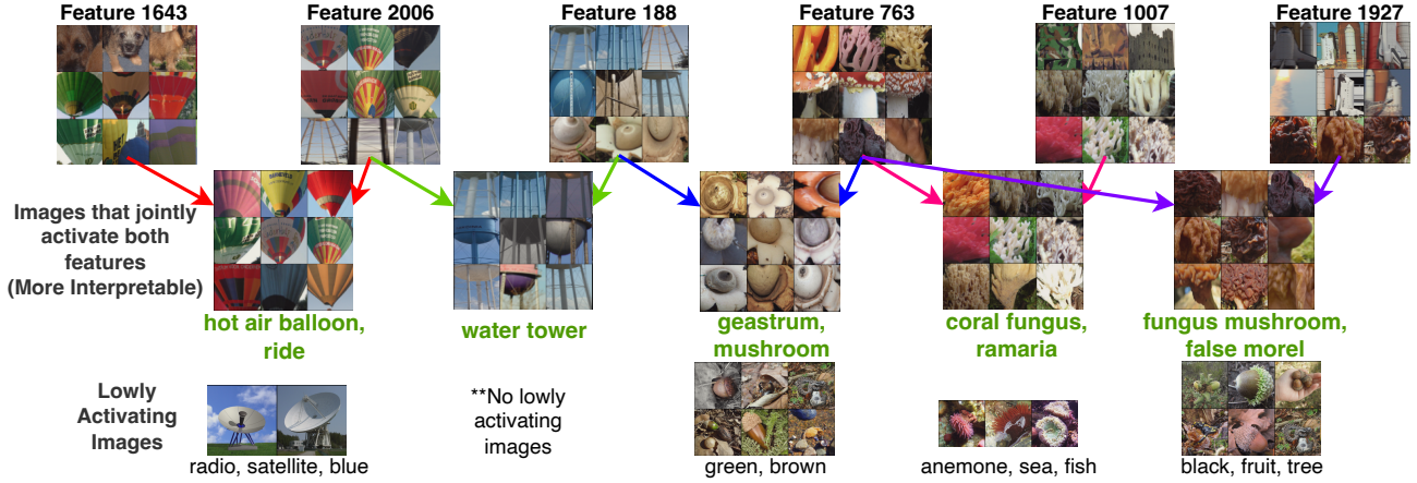
Figure 4. Groups of features can be more interpretable than individual features: In the first panel, we show the highly activating images of some features of DINO (Caron et al., 2021) representations trained on ImageNet (Russakovsky et al., 2015) with a ResNet-50 (He et al., 2016) backbone. We observe that the images are highly diverse with seemingly no shared concept, like “mushrooms” and “water towers” in feature 188. In the second panel, we observe that images that highly activate pairs of features are significantly more connected. The concepts that our framework extracts are strongly correlated to each group of images. For each feature group, we use the lowly activating images (mined from Equation 2) to filter out spurious concepts.
