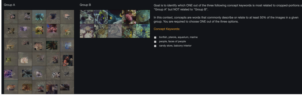
Figure A.5. Amazon Mechanical Turk user study template: A template of our user study where we display two groups of images for a target feature and ask the users to select the best explanation among 3 options.
