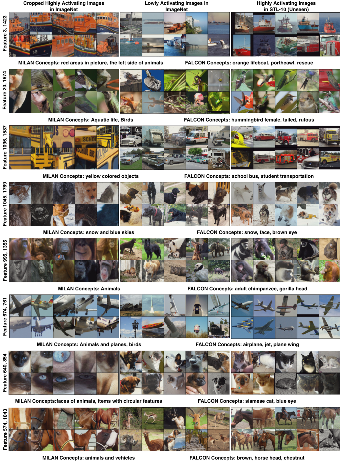
Figure A.7. Generalization of concepts to unseen data: We extract concepts from various features of DINO (Caron et al., 2021) representations (using ImageNet) and verify if they generalize to STL-10 (Coates et al., 2011), an unseen dataset. In all features, the STL-10 images closely resemble the ImageNet images and contain the concepts described by FALCON.
