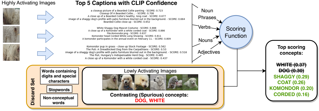
Figure 3. Concept extraction in FALCON using contrasting concepts: We extract a bag of words (nouns, verbs, adjectives) from the top 5 captions (from LAION-400M (Schuhmann et al., 2021)) of every image in the set of highly activating images of a given feature. We use a scoring function (Equation 1) to extract top scoring words and phrases which we refer to as concepts . We also apply contrastive interpretation where we discard any concept that is extracted from the lowly activating images (mined through Equation 2). In this case, “dog” and “white” are spurious concepts that exist in both highly and lowly activating images, implying that they are not discriminative explanations. Therefore, final set of discriminative concepts include “shaggy”, “coat”, “komondor” and “corded” which are all closely related to the given image set.
