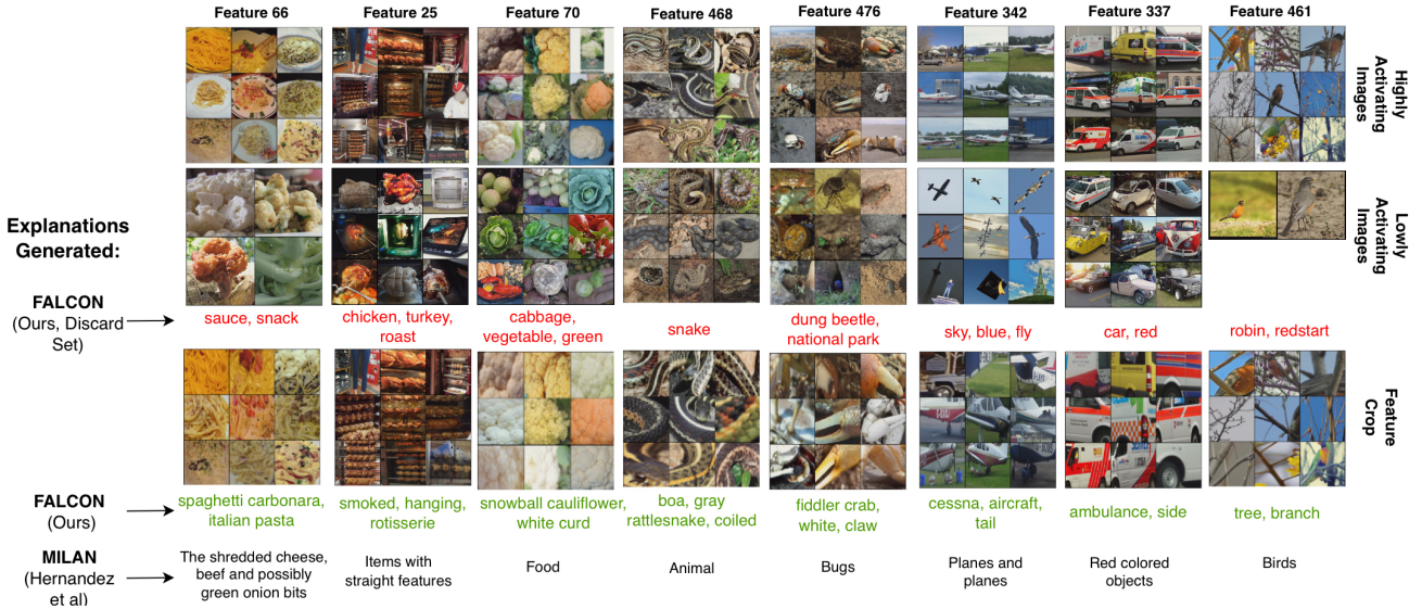
Figure 2. Concepts extracted by FALCON for various features in the SimCLR representation space: We explain various features of the final layer representations of SimCLR (Chen et al., 2020a) pre-trained on ImageNet (Russakovsky et al., 2015) with a ResNet-18 (He et al., 2016) backbone (512 features). For each feature, we show the top activating images as well as the lowly activating images. We crop the top activating images to highlight only the activated regions and extract concepts using the approach outlined in Section 2. The lowly activating images are used to filter spurious concepts using our approach called contrastive interpretation (See Equation 2).
