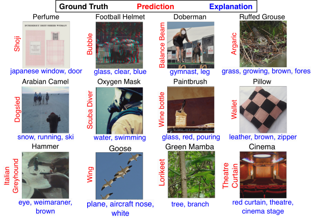
Figure 6. Explaining failures in downstream tasks using concepts: Given SimCLR (Chen et al., 2020a) pre-trained on ImageNet (Russakovsky et al., 2015), we show some mis-classified examples along with the most contributing concepts for their prediction. This allows us to detect and explain concepts which contributed to a model’s decision and help us debug model failures.
