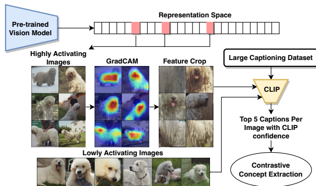
Figure 1. Framework of FALCON: We outline the process of interpreting any given feature(s) in the representation space of a pre-trained model using a probe dataset \mathcal{D} and a captioning dataset \mathcal{S} . Taking the set of highly activating images (from \mathcal{D} ) for the target features we compute their gradient heatmap (Selvaraju et al., 2019) crops, keeping only the highly activating regions. We compute CLIP (Oikarinen & Weng, 2022) image representations of the cropped images and text representations of a large captioning dataset (in our case, LAION-400m (Schuhmann et al., 2021)). For contrastive interpretation , we also caption lowly activating (counterfactual) images. Using cosine similarity, we select the top 5 captions per image and pass them through our concept extraction module (Described in Figure 3).
