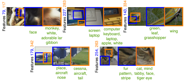
Figure 5. Decomposing images into various concepts: We show some images which highly activate multiple interpretable features. FALCON extracts concepts from feature crops rather than entire images, therefore, each image can be broken down into components, each describing a different physical attribute.
