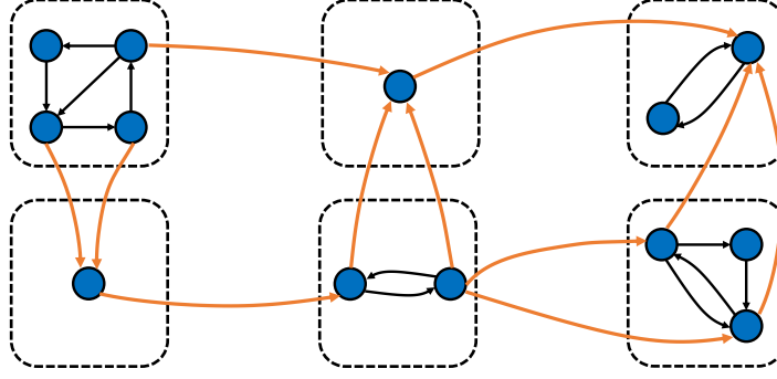
Figure 2: A token-priority graph (TPG) is a directed graph derived from training data (see Sec 2.1 for definition). The edges in TPG capture the input-output relationships between different tokens. A TPG can be partitioned into several SCCs depicted as dashed black squares. In light of Theorem 1, black intra-SCC edges within each SCC induce the soft-composition component of the attention weights whereas the orange edges induce the hard-retrieval component enforcing the priority orders among various SCCs.
