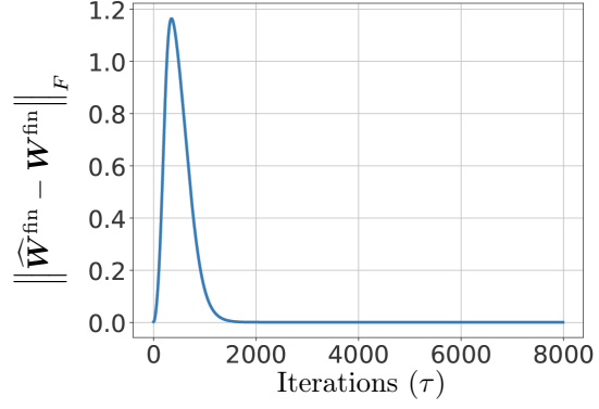
Figure 10: \Pi_{\mathcal{S}_{\text{fin}}}(\mathbf{W}(\tau)) \rightarrow \mathbf{W}^{\text{fin}}
