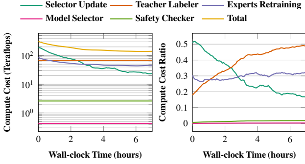
Figure 10: Breakdown of compute cost by the components of RECL controller. The total cost drops over time as the extra-cost of maintaining the model zoo significantly reduces, allowing RECL to enjoy the benefit of model reuse without much additional overhead.
