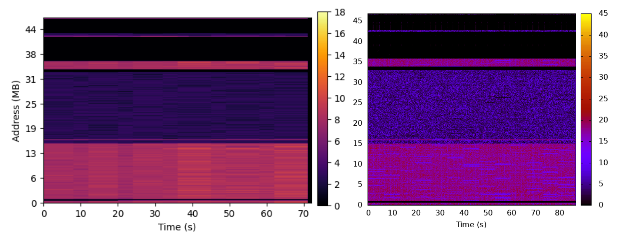
Figure 4. Inferred PyObj temperatures based on refcnt changes.
