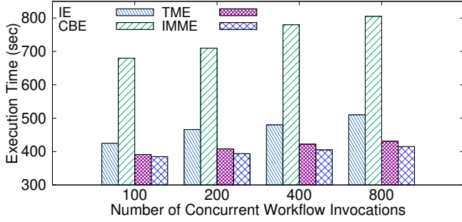
Fig. 11: Impact of our runtime on execution time on an 8-node cluster.
