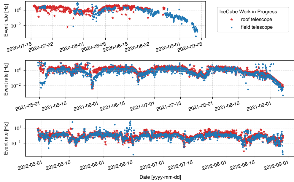
Figure 2: 90-min-averaged event rate for the roof and field telescopes during the three years of operation of IceAct in the current configuration. Each row corresponds to a different data-taking season, split by years.
