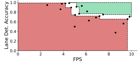
Figure 9: Error constraint space for Polaris-GEM. It captures the interaction of FPS (x-axis) and the errors in the LaneNet model (y-axis). Green region is the valid QoS region, red region is the invalid QoS region, and white regions are unvisited. The black dots on the figure show simulator evaluations.
