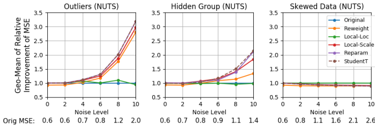
Figure 4: Mean Improvement of Transformed Programs at Different Noise Levels (NUTS)
