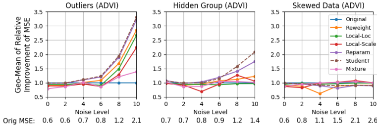
Figure 3: Mean Improvement of Transformed Programs at Different Noise Levels (ADVI)
