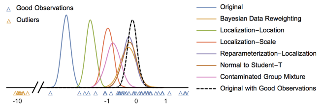
Figure 1: Posteriors of Different Robust Models Fitted with Corrupted Data
