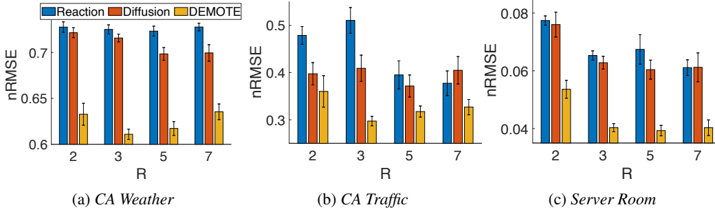
Figure 3: Predictive performance of the diffusion and reaction processes.
