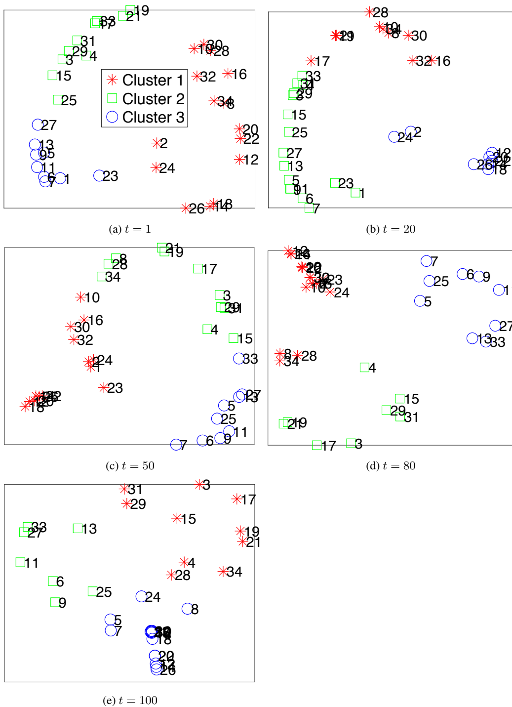
Figure 6: Evolution of the clustering structure within the 34 locations on Server Room dataset.
