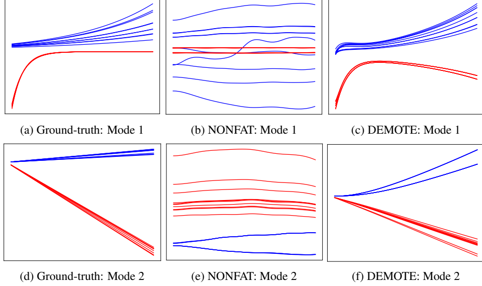
Figure 2: The estimated embedding trajectories for each mode. The color indicates the ground-truth cluster membership.
