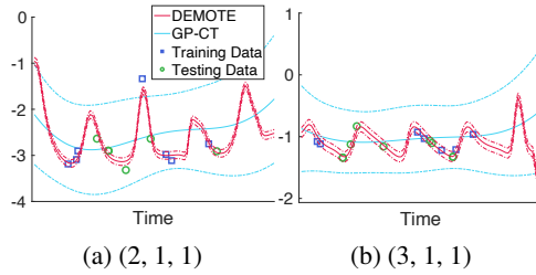
Figure 5: Entry value prediction on Server Room .
