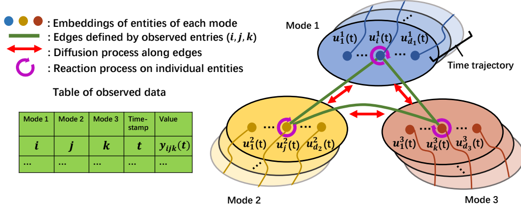
Figure 1: The illustration of the embedding model in DEMOTE.
