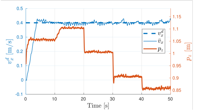
Fig. 7: Generalization of the latent space and trained policy to out-of-distribution data.
