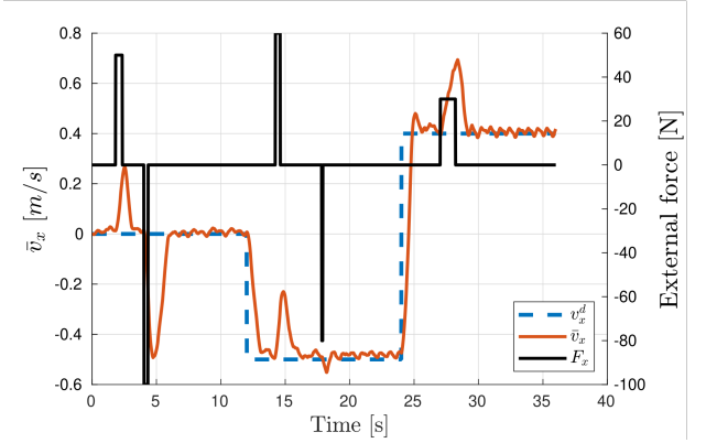
Fig. 8: Robustness test to external disturbances.
