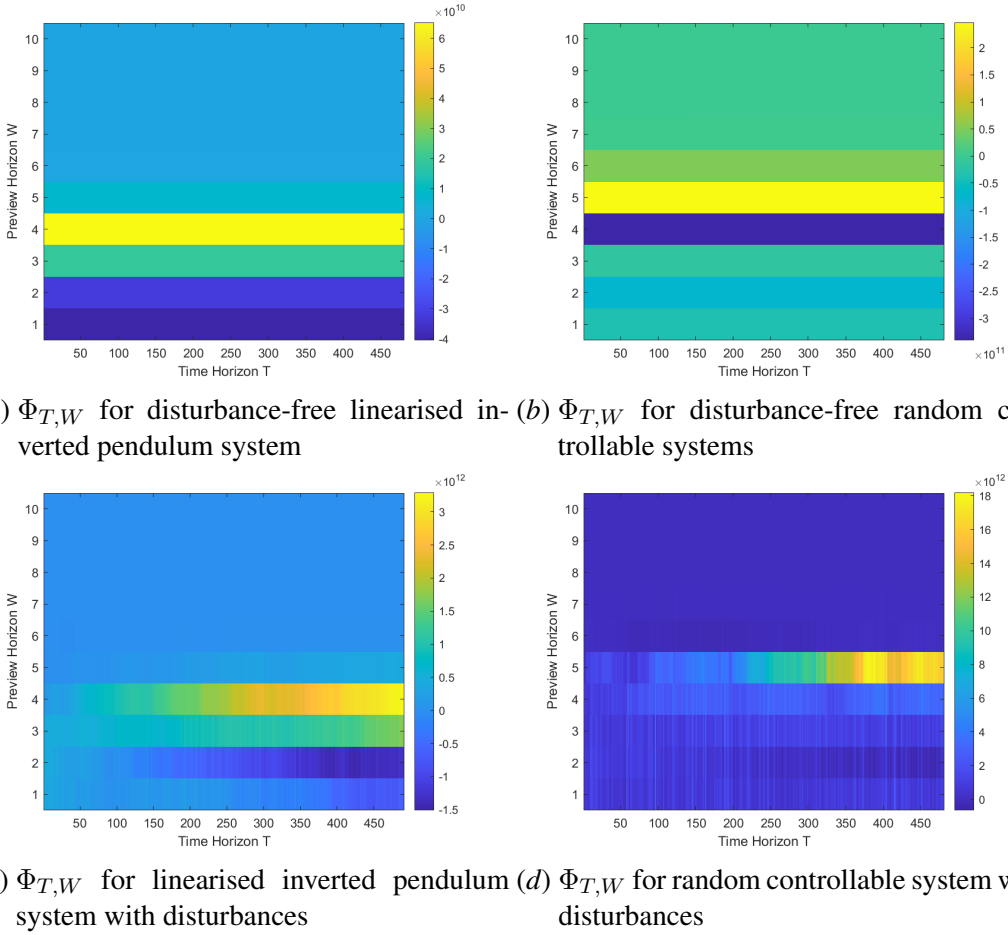
Figure 1: Performance measure \Phi_{T,W} for simulated systems.
