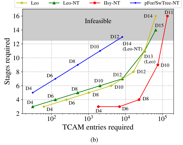
Figure 11: Table entries required to support a programmable class of complete decision trees using SRAM and TCAM. Designs needing more than 12 stages are infeasible on a Tofino switch [8]. Note the logarithm scale on x-axis.
