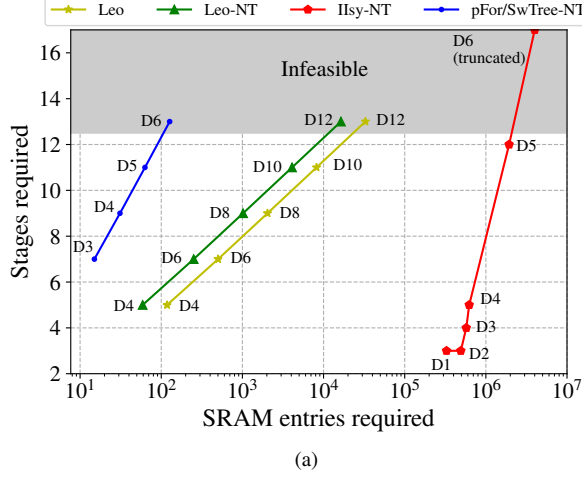
Figure 11: Table entries required to support a programmable class of complete decision trees using SRAM and TCAM. Designs needing more than 12 stages are infeasible on a Tofino switch [8]. Note the logarithm scale on x-axis.
