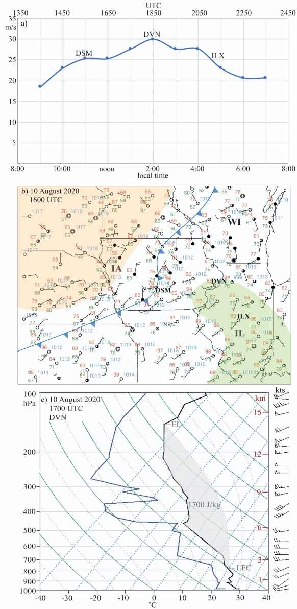
Figure 3. a) Speed of propagation during 1400 UTC 10 August - 0000 UTC 11 August (9 am - 7 pm CDT 10 August) 2020. Approximate arrival times at DSM, DVN, and ILX are indicated. b) Surface station plot for 1600 UTC (11 am CDT) 10 August 2020. The position of the cold front is shown. Dew point temperatures exceeding 75°F are shaded light green, less than 65°F light brown. The locations of Iowa (IA), Wisconsin (WI), and Illinois (IL) are indicated, along with stations DSM, DVN, and ILX (Lincoln, IL). c) National Weather Service special sounding from Davenport, IA (DVN) at 1700 UTC (Noon CDT) on 10 August 10 (about 2 hours before the
