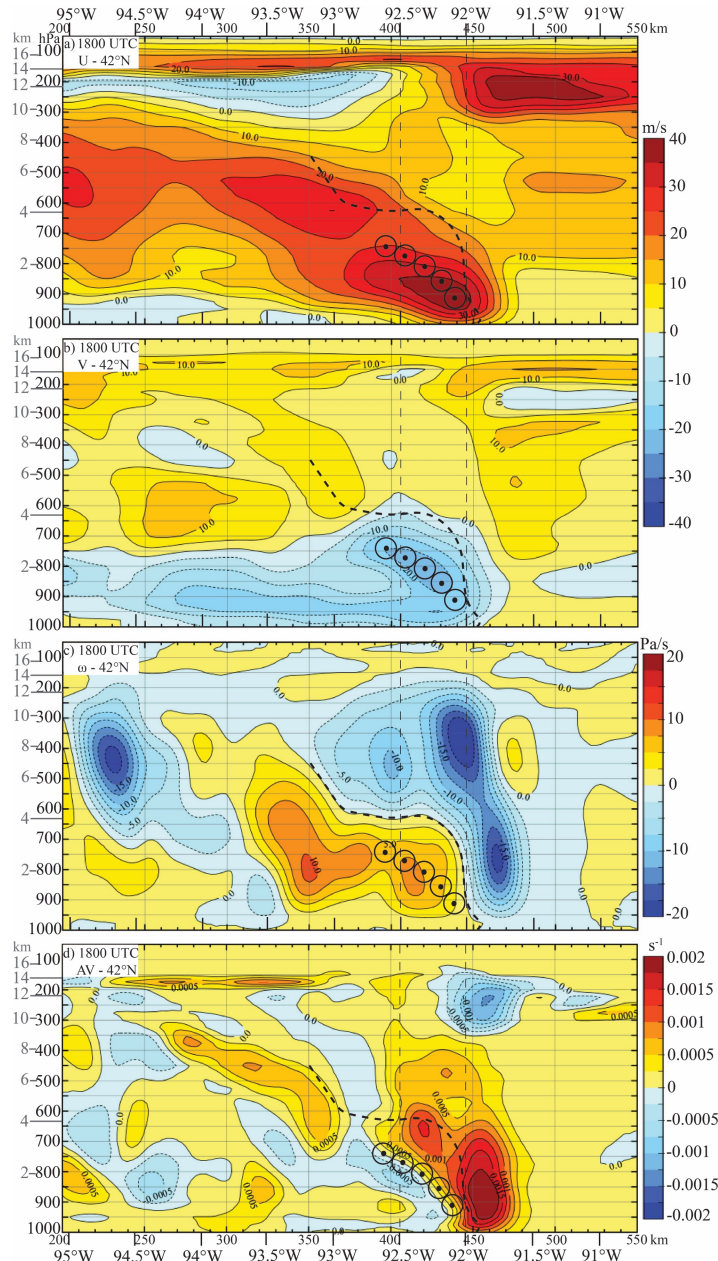
Figure 15. Longitude-altitude sections at 42°N (looking north) of HRRR a) zonal wind (color bar range, interval 5 m/s), b) meridional wind (color bar, interval 5 m/s), c) pressure velocity (color bar, interval 2.5 Pa/s), and d) absolute vorticity (color bar, interval 0.00025 s -1 ) at 1800 UTC 10 August 2020. The zero vertical velocity line (heavy dashed) and locations of updrafts and downdraft (arrows) in c) are transposed onto a), b), and d). The locus of southward flow in b) is indicated with outward arrow symbols (⊙) and transposed onto a), c), and d). Distance east of the center of the HRRR domain (km) is shown along the x-axis. Pressure (hPa) and altitude (km, gray tick marks) are shown on the y-axis.
