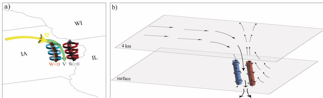
Figure 1. Idealized 3D representation in the lower troposphere of the relationship between a) the westerly inflow jet (yellow), northerly surface outflow jet (green arrow), lower-tropospheric PV dipole (blue/negative and red/positive), downdraft (brown arrow), and updraft (black arrow), and b) perspective view showing the air mass pathways, with horizontal reference planes near the surface and 4 km altitude.
