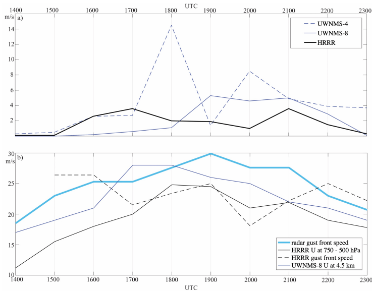
Figure 7. Hourly time series during the period 1400 – 2300 UTC 10 August 2020 of a) maximum updraft velocity (m/s) along 42^{\circ}\text{N} at 700 hPa for HRRR (thick black), and at 3.18 km altitude for UWNMS-4 (dashed blue), and UWNMS-8 (blue) simulations and b) radar gust front speed from Fig. 3a (m/s, thick blue), HRRR zonal wind speed 100 km upstream of the gust front averaged in the layer 500-700 hPa (black), gust front speed estimated from HRRR surface wind pattern (dashed black), and UWNMS-8 zonal wind speed at 4.5 km altitude 50 km upstream and 50 km poleward of the gust front (blue).
