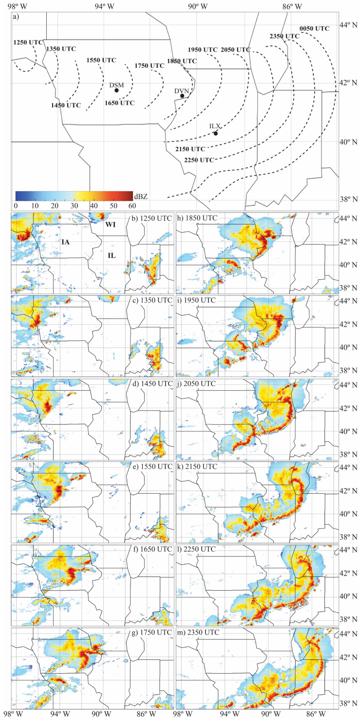
Figure 2. a) Progression of the arc of high reflectivity from 1250 UTC 10 August to 0050 UTC 11 August 2020 (7:50 am to 8:50 pm CDT 10 August). Panels b) - m) show hourly snapshots from 1250 to 2350 UTC. The locations of Des Moines, IA (DSM), Davenport, IA (DVN), and Lincoln, IL (ILX) are indicated in panel a). Values of dBZ less than zero are not plotted.
