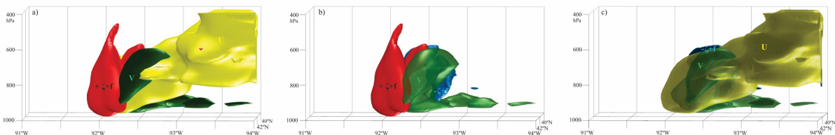
Figure 19. HRRR 3D isosurfaces for 1800 UTC 10 August 2020 viewed from the north of a) u = 23 m/s (yellow), v = -18 m/s (green), and \zeta + f = 10 \times 10^{-4} \text{ s}^{-1} (red), b) v = -18 m/s (green), \zeta + f = 10 \times 10^{-4} \text{ s}^{-1} (red), and \zeta + f = -7 \times 10^{-4} \text{ s}^{-1} (blue), and c) u = 23 m/s (yellow), v = -18 m/s (green), and \zeta + f = -7 \times 10^{-4} \text{ s}^{-1} (blue).
