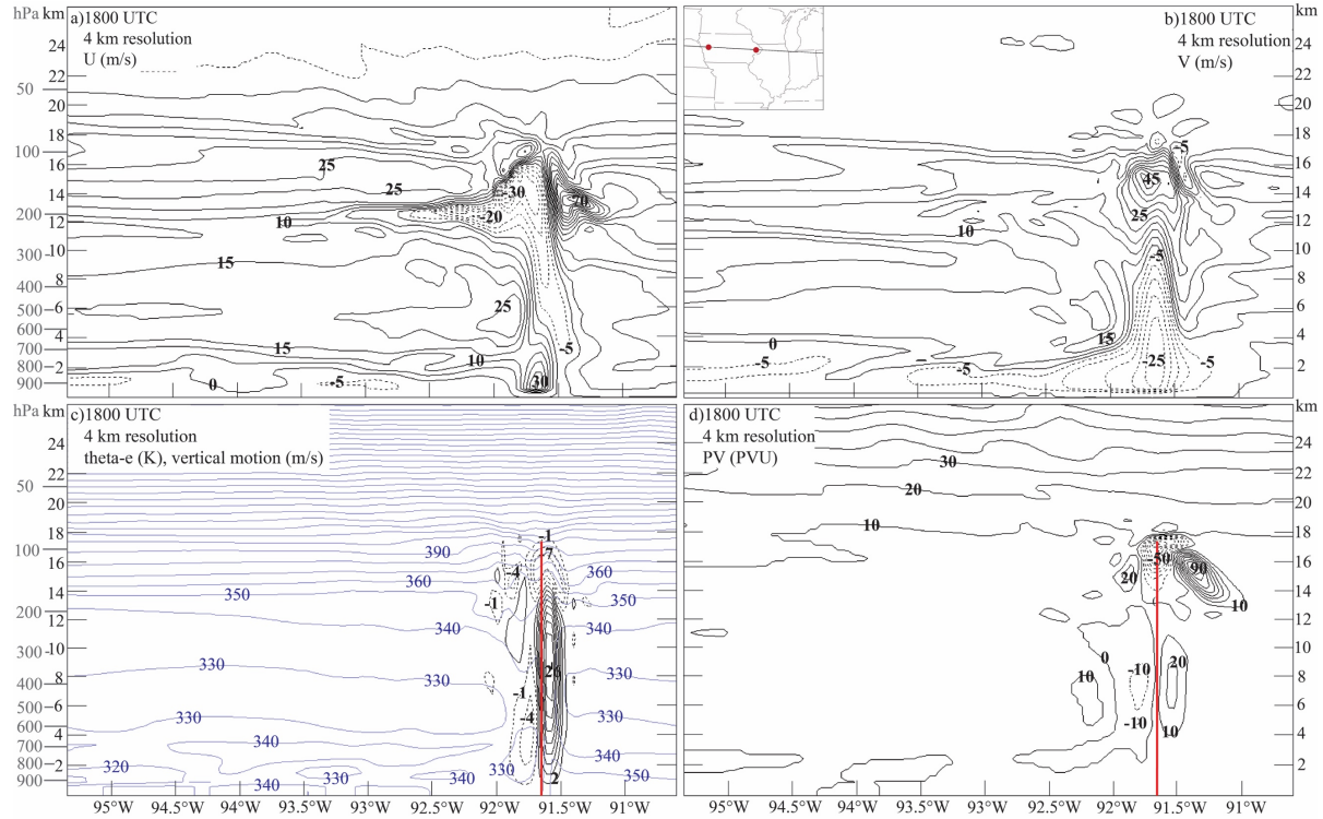
Figure 9. Longitude-altitude sections in UWNMS-4 at 1800 UTC 10 August 2020 for a) zonal wind (contour interval 5 m/s, negative dashed), b) meridional wind (contour interval 5 m/s, negative dashed), c) equivalent potential temperature (blue contours, interval 10 K) and vertical wind (contour interval 3 m/s, negative dashed), and d) PV (contour interval 10 PVU, negative dashed). The vertical line in each panel indicates the longitude of maximum northerly flow in b). The location of this section is shown in the inset of panel b).
