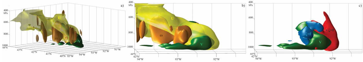
Figure 18. HRRR 3D isosurfaces for 1800 UTC 10 August 2020 of a) u = 23 m/s (yellow), v = -18 m/s (green), and \omega = 6 Pa/s (orange) viewed obliquely from the southwest, b) as in a) except viewed from the south, and c) v = -18 m/s (green), \zeta + f = 10 \times 10^{-4} \text{ s}^{-1} (red), and \zeta + f = -7 \times 10^{-4} \text{ s}^{-1} (blue) viewed from the south.
