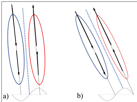
Figure 20. Idealized diagram showing the maxima in diabatic stretching tendency for a) weak tilt and b) strong tilt. The downdraft (convergent arrows) coincides with negative PV anomaly (blue), the updraft (divergent arrows) coincides with positive PV anomaly (red), with a northerly jet between (dotted blue axis). With increasing tilt, the maxima in diabatic stretching tendency,
