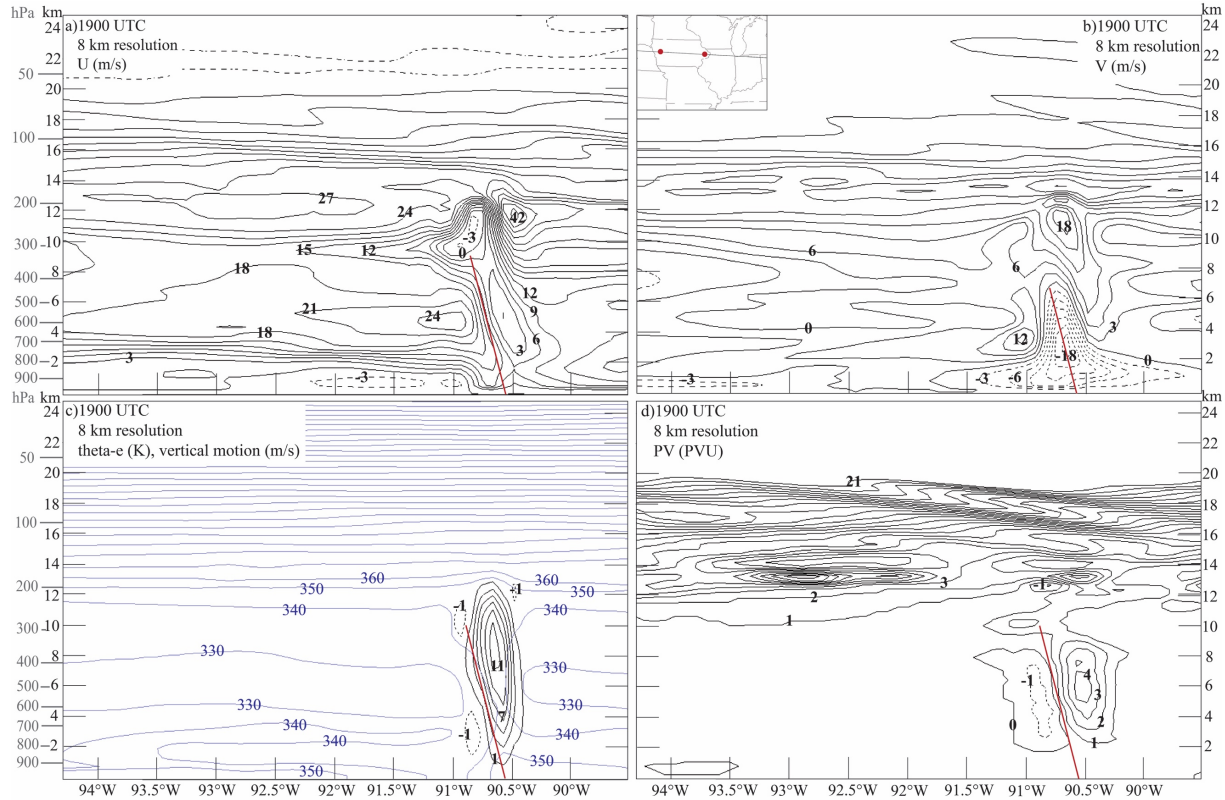
Figure 10. Longitude-altitude sections in UWNMS-8 at 1900 UTC 10 August 2020 for a) zonal wind (contour interval 3 m/s, negative dashed), b) meridional wind (contour interval 3 m/s, negative dashed), c) equivalent potential temperature (blue contours, interval 10 K) and vertical wind (contour interval 2 m/s, negative dashed), and d) PV (contour interval 1 PVU, negative dashed). The tilted vertical line in each panel indicates the axis of maximum northerly wind.
