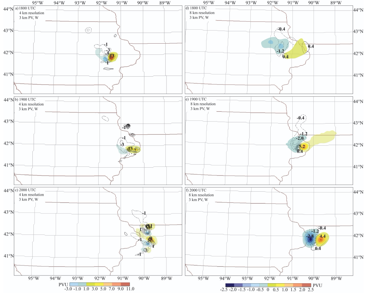
Figure 8. Plan views of PV (color bar) and vertical velocity (m/s, contours, negative dashed) at 3 km altitude for UWNMS-4 (left) and UWNMS-8 (right) for a), d) 1800 UTC, b), e) 1900 UTC, and c), f) 2000 UTC 10 August 2020. In UWNMS-4 vertical velocity is contoured every 2 m/s and PV every 2 PVU, while in UWNMS-8 vertical velocity is contoured every 0.8 m/s and PV every 0.5 PVU.
