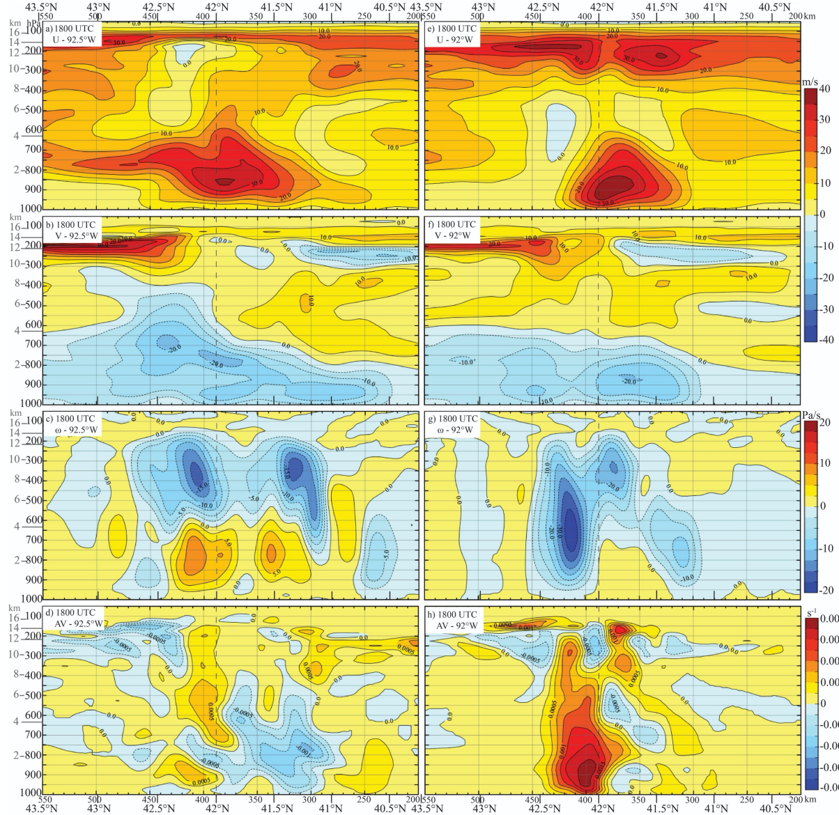
Figure 16. Latitude-altitude sections (eastward view) at 92.5°W (left) and 92°W (right) of HRRR a) zonal wind (color bar range, interval 5 m/s), b) meridional wind (color bar, interval 5 m/s), c) pressure velocity (color bar, interval 2.5 Pa/s), and d) absolute vorticity (color bar, interval .00025 s -1 ) at 1800 UTC 10 August 2020. The dashed vertical line shows 42°N, the latitude of sections in Fig. 8. Distance north of the center of the HRRR domain is shown in km. Pressure (hPa) and altitude (km, gray tick marks) are shown on the vertical axis.
