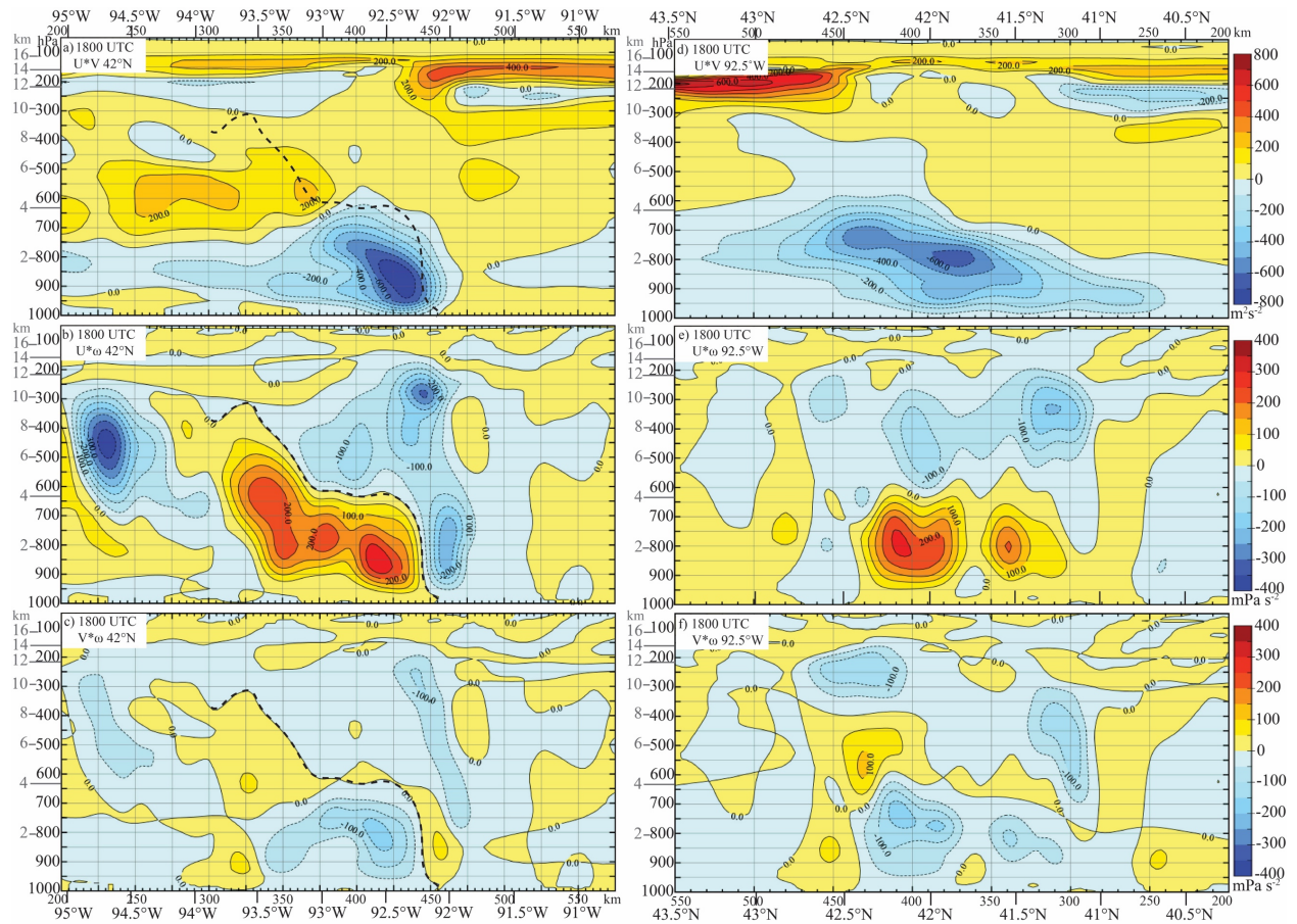
Figure 17. Reynolds stresses u \cdot v (top, color bar, interval 100 \text{ m}^2 \text{s}^{-2} ), u \cdot \omega (middle, color bar, interval 50 \text{ mPa s}^{-2} ), and v \cdot \omega (bottom, color bar, interval 50 \text{ mPa s}^{-2} ) in HRRR for longitude-altitude sections at 42°N looking north (a, b, c) and for a latitude-altitude section at 92.5°W looking east (d, e, f). The zero vertical wind line in Fig. 15c) is transposed onto panels a), b), and c). At left, both longitude and distance (km) east of the center of the HRRR domain are shown. At right, both latitude and distance north of the center of the HRRR domain are shown. Pressure (hPa) and altitude (km, gray tick marks) are shown on the vertical axis.
