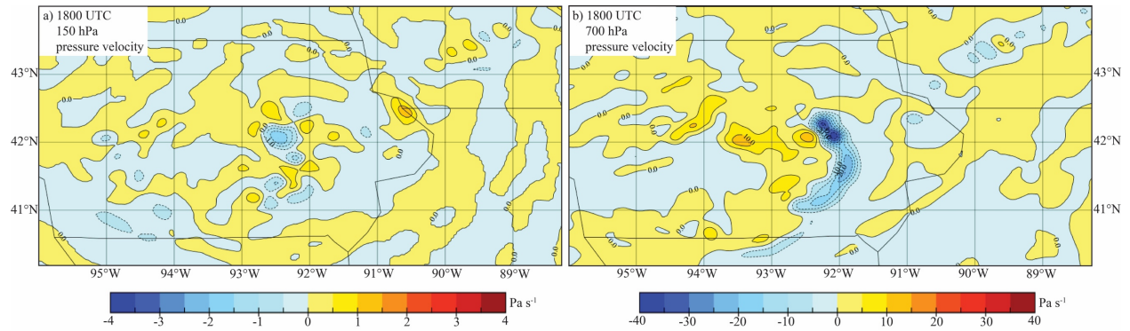
Figure 14. HRRR pressure velocity (color bar, interval 0.5 Pa/s) at 1800 UTC on 10 August 2020 for a) 150 hPa and b) 700 hPa.
