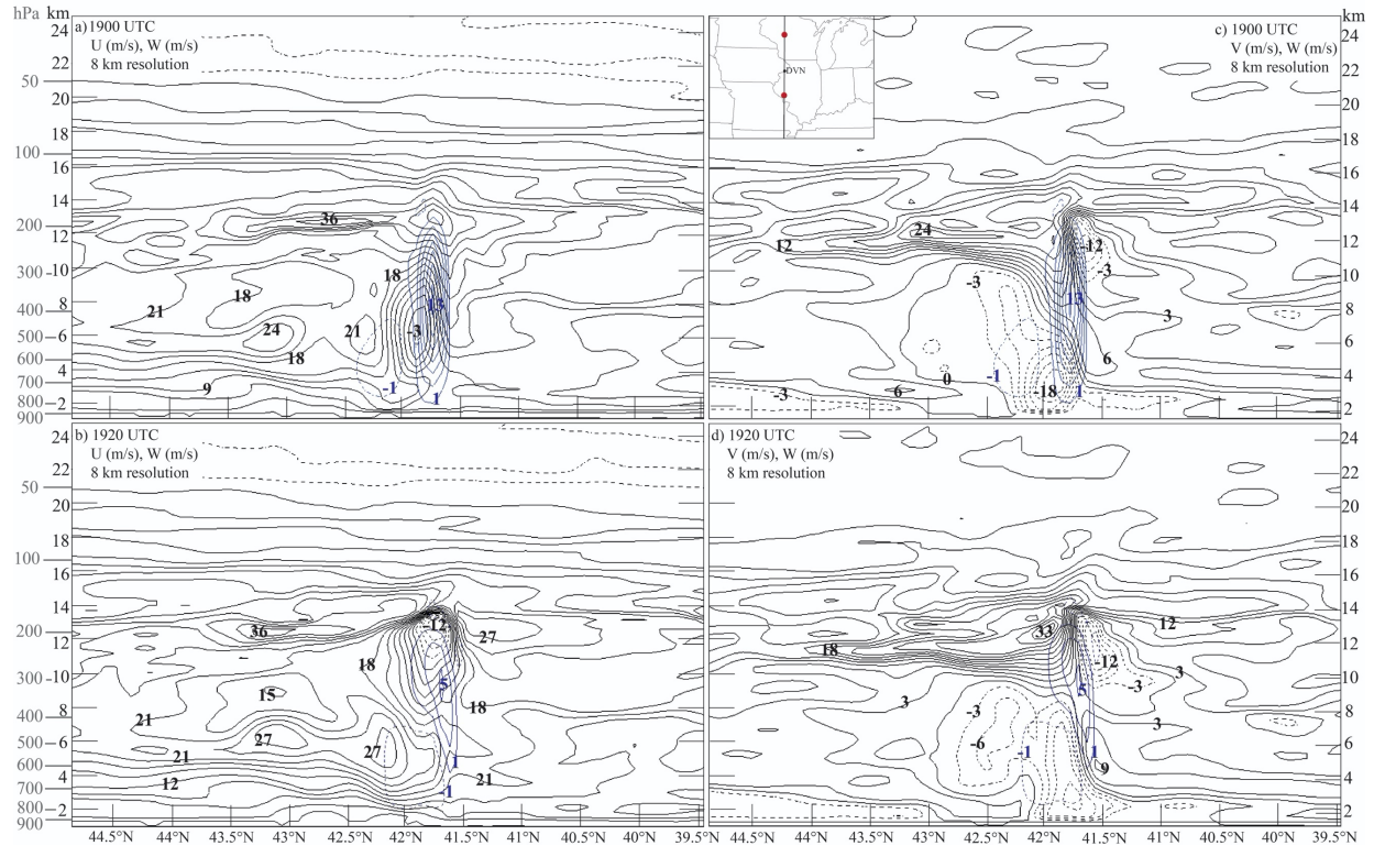
Figure 11. Meridional sections along 90.58°W of UWNMS-8 (left) zonal wind and (right) meridional wind (black contours every 3 m/s, negative dashed), with vertical wind (blue contours every 2 m/s, negative dashed) at (top) 1900 and (bottom) 1920 UTC on 10 August 2020. The view is toward the east, with north to the left. The locations of the section ends (dots) are shown in the inset.
