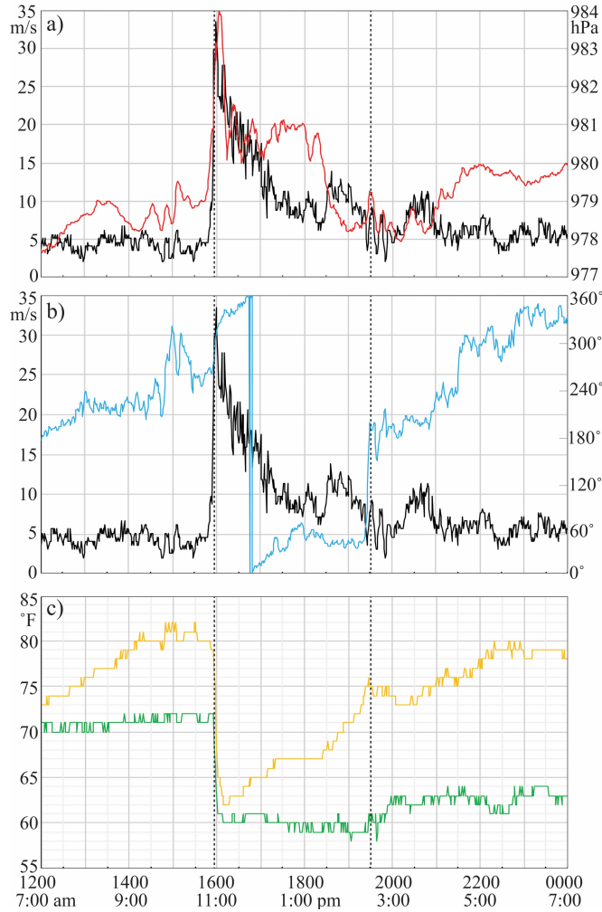
Figure 5. Iowa Environmental Mesonet surface meteorological observations at Des Moines, Iowa (DSM) during 1200 – 2400 UTC (7 am – 7 pm CDT) 10 August 2020 of a) surface pressure (red line) and gust speed (black), b) gust speed (black) and wind direction (blue), and c) temperature (yellow) and dew point temperature (green). Data are shown at 1-min intervals. Vertical dashed lines indicate the duration of the cold pool at DSM.
