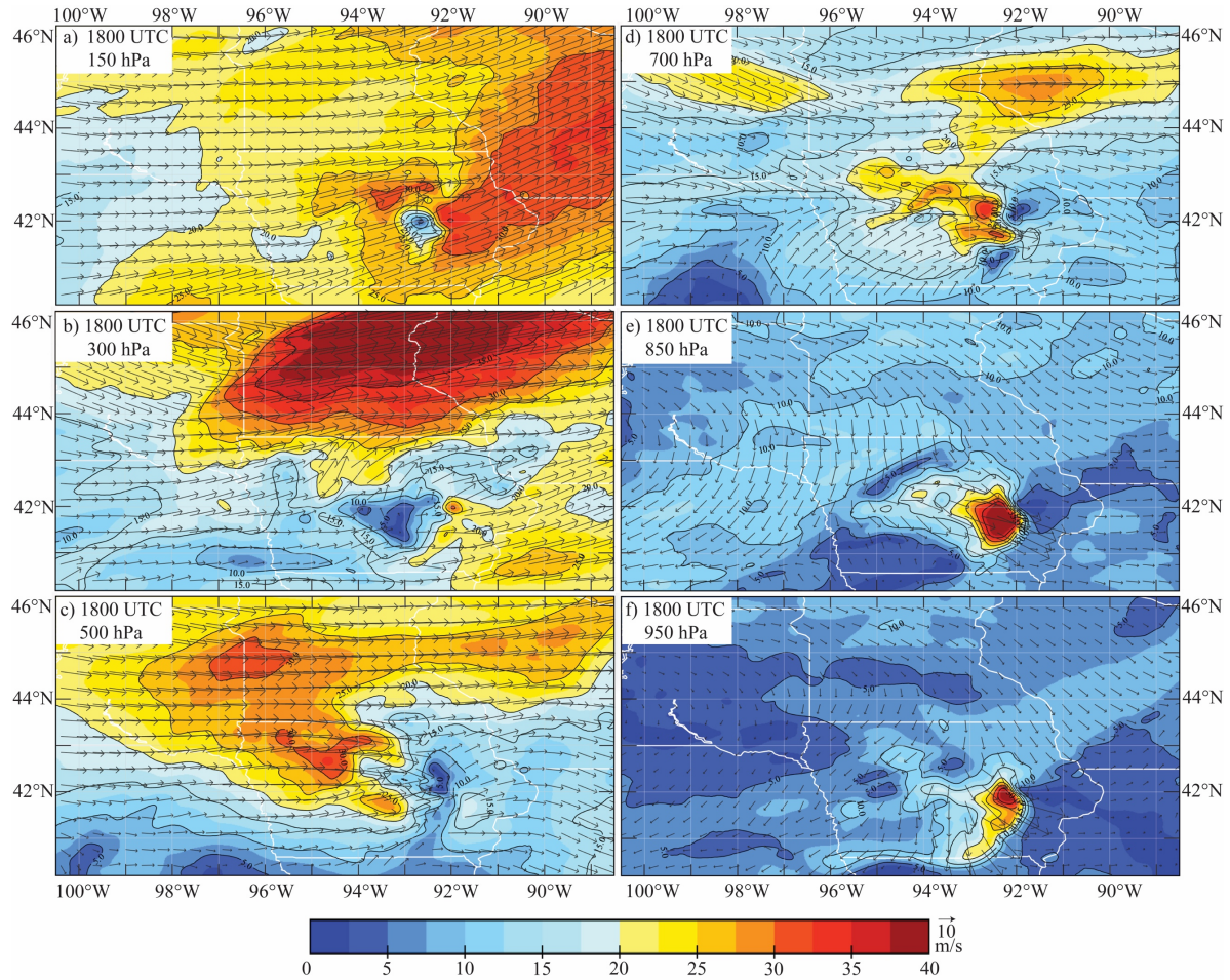
Figure 6. HRRR horizontal wind speed (color bar, interval 2.5 m/s) and wind vectors (reference length 10 m/s) at 1800 UTC on 10 August 2020 for a) 150 hPa, b) 300 hPa, c) 500 hPa, d) 700 hPa, e) 850 hPa, and f) 950 hPa.
