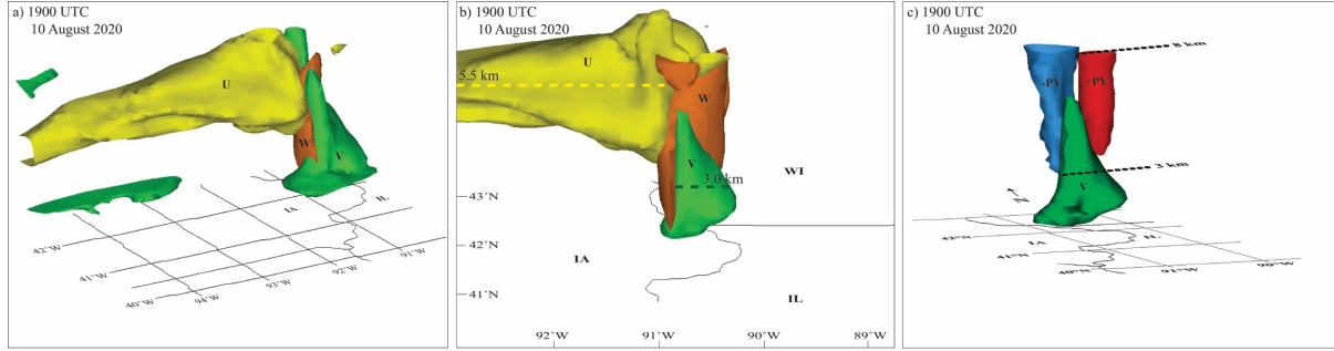
Figure 12. Spatial relationship between the westerly inflow jet, lower-tropospheric northerly jet, and the downdraft in UWNMS-8 at 1900 UTC 10 August 2020. Perspective views from a) the southwest and b) south showing isosurfaces of zonal wind (U, 22 m/s, yellow), meridional wind (V, -5 m/s, green), and vertical wind (W, -0.8 m/s, orange), and c) from the southwest showing an isosurface of meridional wind (V, -5 m/s, green), together with the -1 PVU (blue) and +2 PVU (red) isosurfaces. Selected altitudes are indicated in b) and c).
