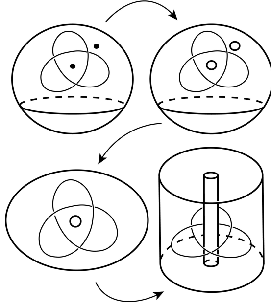
FIGURE 7. A staked link L_D \subset S^2 with n stakes determines a link \bar{L}_D in a handlebody of genus n - 1 .
