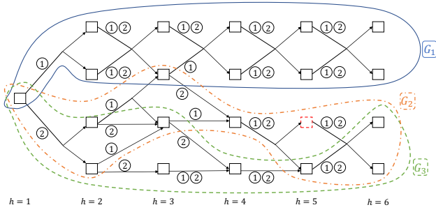
Figure 1. A sketch of subgraph examples. Squares represent states. The red dashed square at step h = 5 is the unsafe state. Circles represent actions. Arrows represent state transitions. There are two actions a = 1, 2 , as shown by the numbers in the circles.
