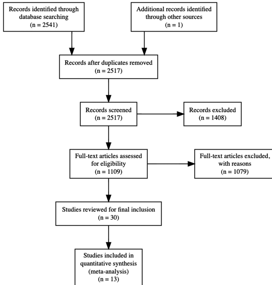
Figure 1 PRISMA Flowchart
