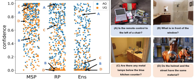
Figure 8: Left: confidence scores of MSP, RP, and Ens methods for 500 random samples. Right: qualitative examples. AQs/UQs are shown in blue/orange. B is an annotation error in the original GQA dataset.
