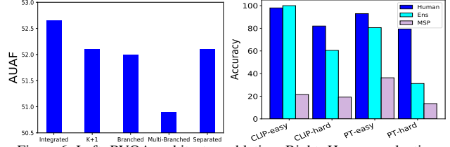
Figure 6: Left: RVQA architecture ablation. Right: Human evaluation.
