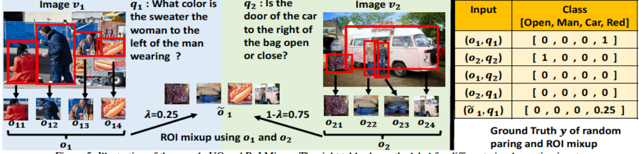
Figure 5: Illustration of the pseudo UQ and RoI Mixup. The right table shows the label for different visual question inputs.
