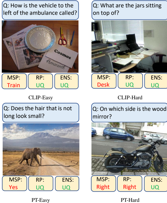
Figure 7: Qualitative examples for a threshold such that all models achieve 55% accuracy.
