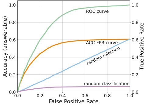
Figure 4: Comparison between ROC curve (green; right axis) and ACC-FPR curve (orange; left axis). See text for details.
