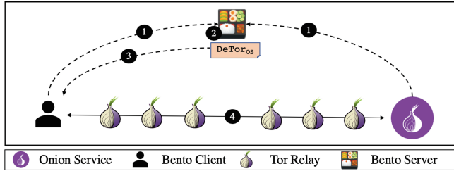
Fig. 2. The DeTor OS Protocol for never-once and never-twice avoidance. Both parties send their circuit information to a Bento server which is running the DeTor OS function. The server then computes the desired avoidance proof and sends it to the client. If successful, the client then begins communicating with the onion service.
