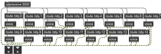
Figure 8: The MaxPy-generated abstraction [yag-voices], containing a variable number of voices connected to OSC triggers.
