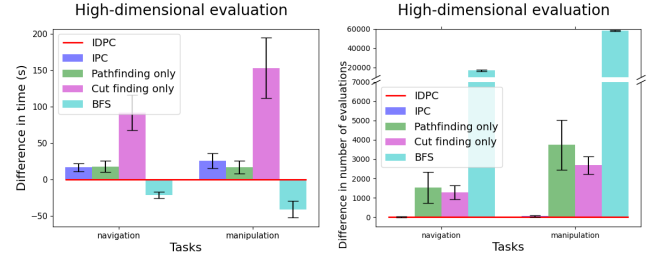
Fig. 13. Plots comparing the results for navigation and manipulation tasks. For the navigation task, PRM generates a roadmap consisting of 5000 vertices with 20000 edges. The roadmap includes 10000 vertices with 60000 edges for the manipulation task.
