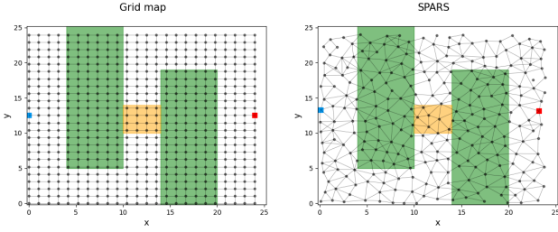
Fig. 15. Depiction of the graph topologies when using different roadmap types. The detailed explanation of the figures can be found in Figure 9. The left figure shows a grid map example used for search-based planning, and the right figure shows a roadmap example generated by SPARS used for sampling-based motion planning.
