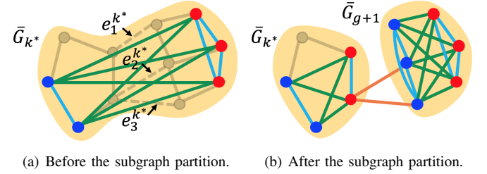
Fig. 8. Depiction of the subgraph partition process. The meaning of colors used for vertices and edges is the same as in Figure 6. The candidate cut applied in this example is C_{k^*} = \{e_1^{k^*}, e_2^{k^*}, e_3^{k^*}\} ( i.e. , dotted lines in (a)), where e_1^{k^*} is in-collision while e_2^{k^*} and e_3^{k^*} are collision-free.
