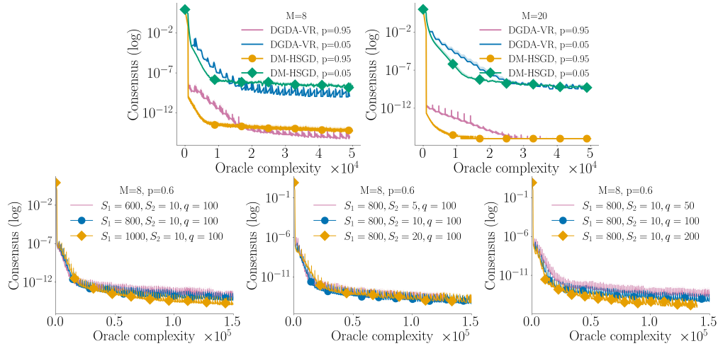
Figure 2: Sensitivity analysis results for the PL game (13). The first two plots show the sensitivity analysis in terms of graph connectivity \rho , while the last three show the sensitivity analysis in terms of the batchsizes S_1, S_2 and the frequency q . Here, oracle complexity refers to data points visited.
