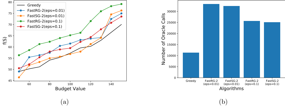
Figure 4: A comparison of objective value and runtime of Greedy, Repeated Greedy, and Simultaneous Greedys for problem instances in Experiment 2. The linear time and knapsack variants of Repeated Greedy and Simultaneous Greedys are displayed here. Fig 4a plots the objective values attained by the algorithms against the budget value. Fig 4b plots the number of oracle calls for budget value \beta = 150
