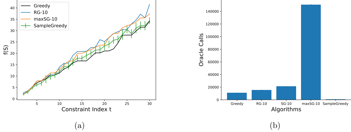
Figure 2: A comparison of objective value and runtime of Greedy, Sample Greedy, Repeated Greedy, and Simultaneous Greedys for problem instances in Experiment 1. Linear time implementations with \varepsilon \in \{0.1, 0.01\} were run, but not reported here because the execution path did not change. Fig 2a plots the objective value attained by the algorithms against the constraint index. Fig 2b plots the number of oracle calls for index t = 30 .
