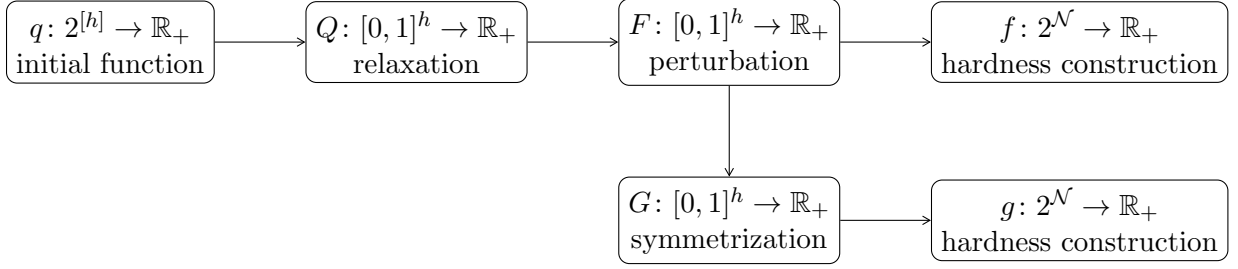
Figure 1: Construction of the objective functions f and g .
