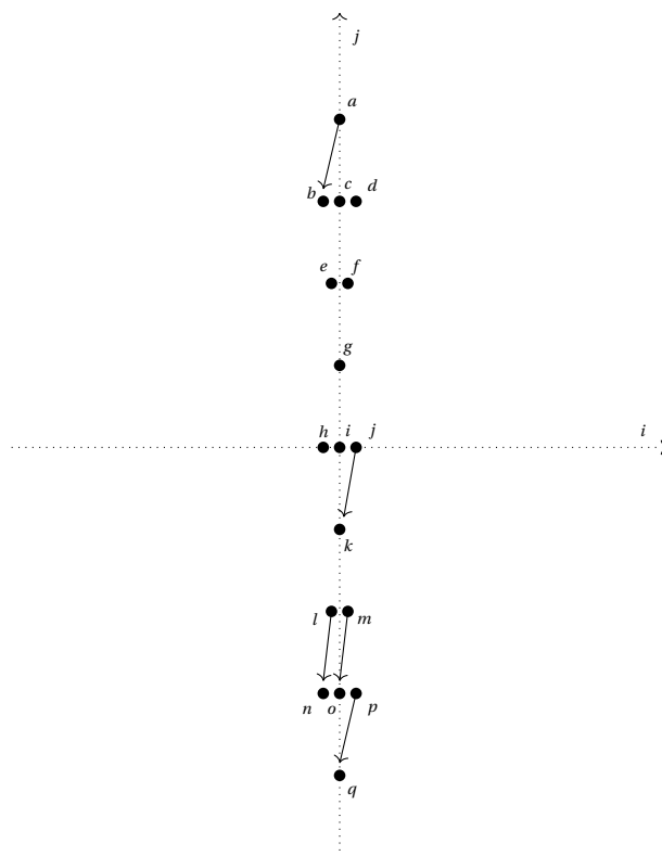
Figure 21: An incomplete picture for CFK^\infty(11n_{57}) with part of \partial_{\text{vert}} denoted by the arrows. Here \partial(c) = 0 and the vertical differentials of the remaining unpaired elements are not yet determined.
