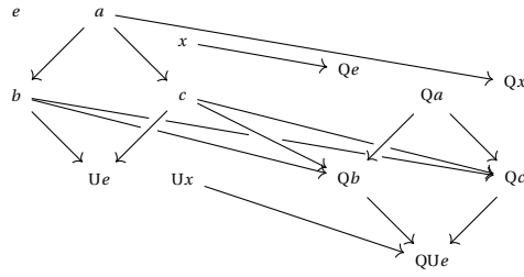
Figure 13: AI_0^- for the figure eight knot consists of the structure shown, and all positive U -translates of the generators a, b, c, x, Ux, Ue, Qa, Qb, Qc, Qx , and QUe .
