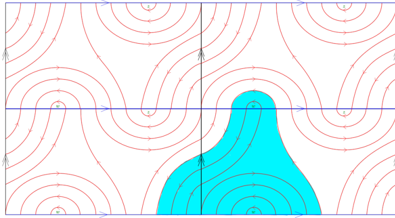
Figure 32: The disk highlighted in blue is a bigon from x_{-5} to x_{-3} containing two copies of w ; the corresponding arrow in the chain complex runs from x_{-5} to U^2 x_{-3} .
