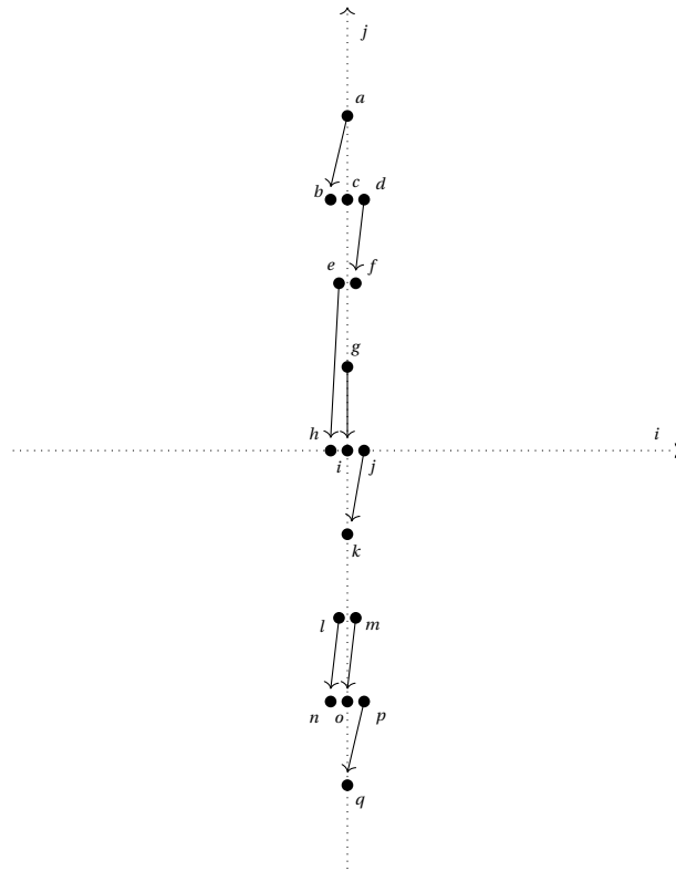
Figure 23: An updated, and now complete picture of C\{i = 0\} . All generators are paired up by the vertical differential, except for c , which generates the homology of the complex.
