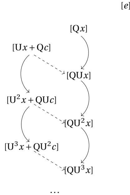
Figure 15: H_*(AI_0^-) for the figure eight knot can be described by two linked towers and the stand-alone subspace [e] .
