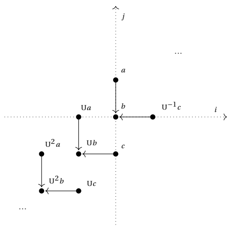
Figure 5: The chain complex \text{CFK}^{\infty}(\overline{3_1}) has three generators, which we call a , b , and c . The homological grading of a is 2; b has homological grading 1; and c has homological grading 0.
