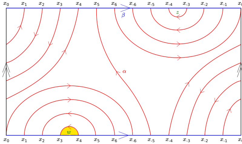
Figure 31: The disk highlighted in yellow is a bigon from x_4 to x_3 containing one copy of w ; the corresponding arrow in the chain complex runs from x_4 to Ux_3 .
