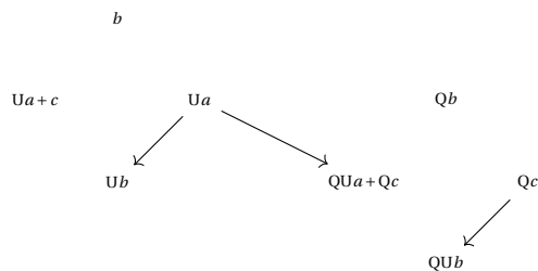
Figure 11: The simplified mapping cone for the left handed trefoil.
