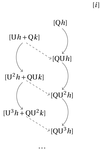
Figure 29: H_*(AI_0^-) for the knot 11n_{57} can be described by two linked towers and the stand-alone subspace [i] .
