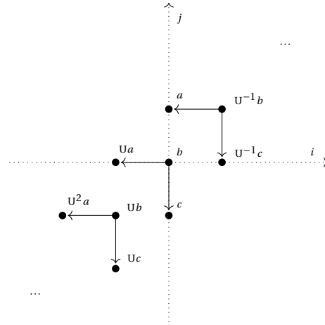
Figure 4: The chain complex CFK^\infty(3_1) has three generators, which we call a, b , and c . The arrows in the picture represent the boundary map \partial . The homological grading of a is 0; b has homological grading -1; and c has homological grading -2.
