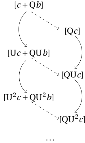
Figure 9: H_*(AI_0^-) for the right-handed trefoil knot can be described by two linked towers. The tower on the left contains no elements in the image of Q , while the tower on the right contains only elements that are in the image of Q . Each tower is organized by increasing powers of U . Curved lines denote multiplication by U , while dashed lines denote application of Q .
