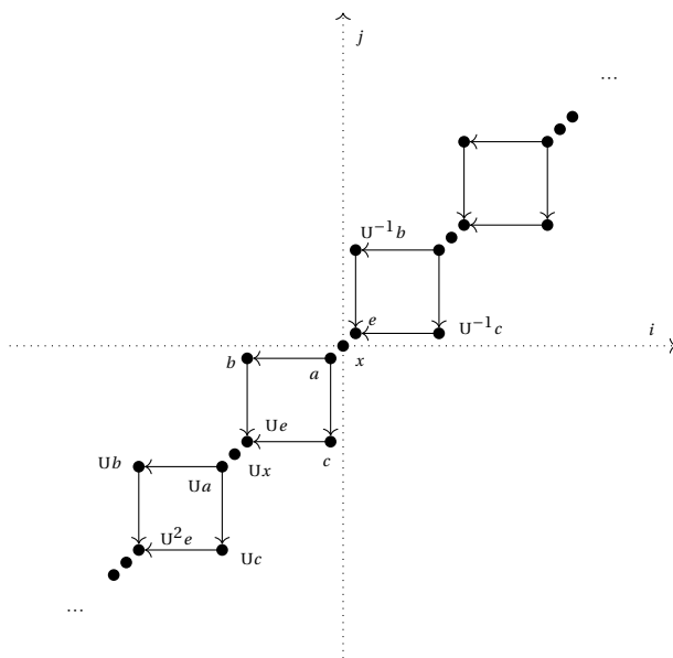
Figure 6: The chain complex \text{CFK}^{\infty}(4_1) has five generators, which we call a , b , c , e and x . The homological gradings of a , e and x are 0; b has homological grading 1; and c has homological grading -1.
