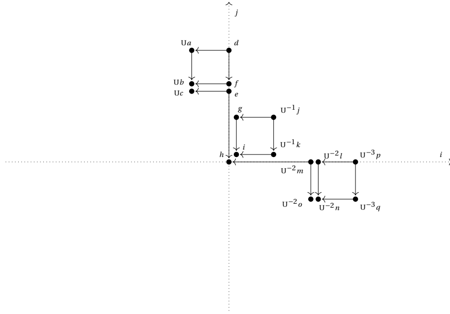
Figure 25: CFK^\infty(11n_{57}) decomposes as an \mathbb{F}_2[U, U^{-1}] complex into the direct sum of a staircase and three boxes.
