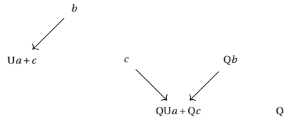
Figure 8: AI_0^- for the right-handed trefoil knot shown after applying a change of basis to the structure in Figure 7.
