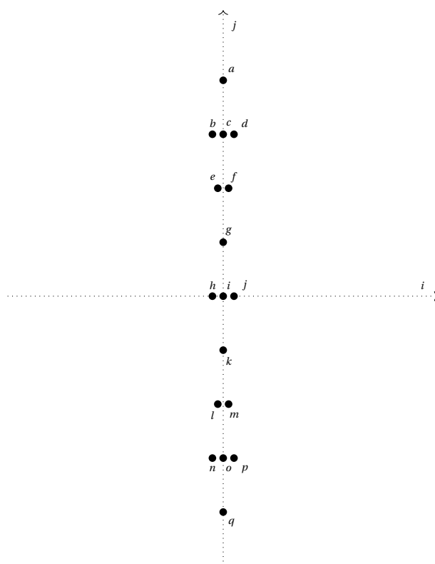
Figure 20: Arrangement of generators of CFK^\infty(11n_{57}) . The homological grading of a is 1; b, c , and d are in homological grading 0; e, g , and g are in homological grading -1 ; h, i , and j are in homological grading -2 ; k is in homological grading -3 ; l and m are in homological grading -5 ; n, o , and p are in homological grading -6 ; q has homological grading -7 .
