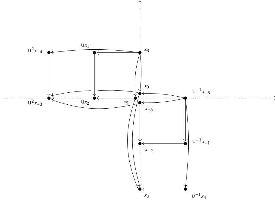
Figure 33: CFK^\infty(10_{161}) prior to a change of basis.
