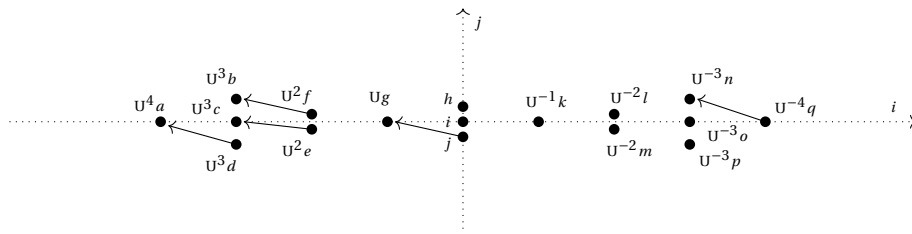
Figure 24: An updated, but incomplete picture for C\{j = 0\} with the horizontal differential of U^3 d, U^2 e, U^2 f, j , and U^{-4} q denoted by the arrows.
