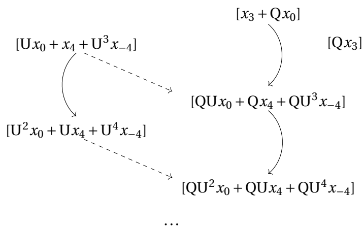
Figure 35: H_*(AI_0^-) for the knot 10_{161} can be written as two towers related by the action of Q and the stand-alone subspace [Qx_3] .
