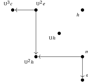
Figure 26: A_0^- for the staircase subcomplex of CFK^\infty(11n_{57}) consists of all non-negative U -translates of the staircase shown, along with the elements h and Uh .
