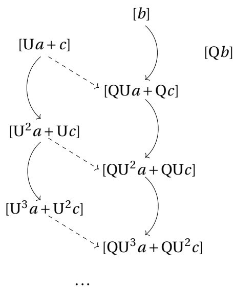
Figure 12: H_*(AI_0^-) for the left handed trefoil knot can be described by two linked towers and the stand-alone subspace [Qb] . Note that QUb is in the image of the differential.
