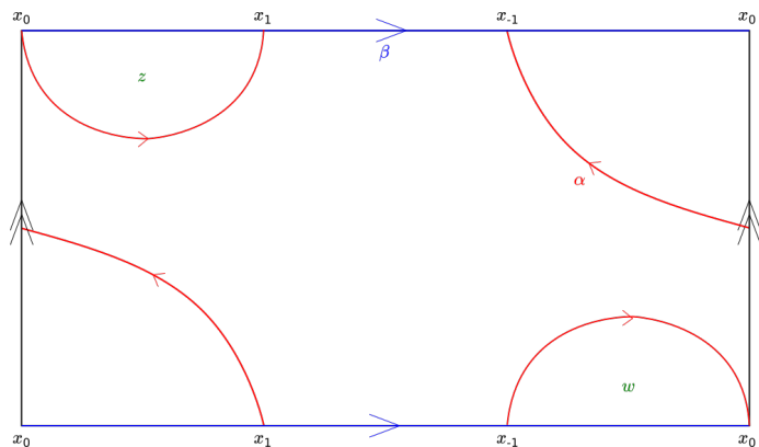
Figure 17: The Heegaard diagram for the right-handed trefoil knot.
