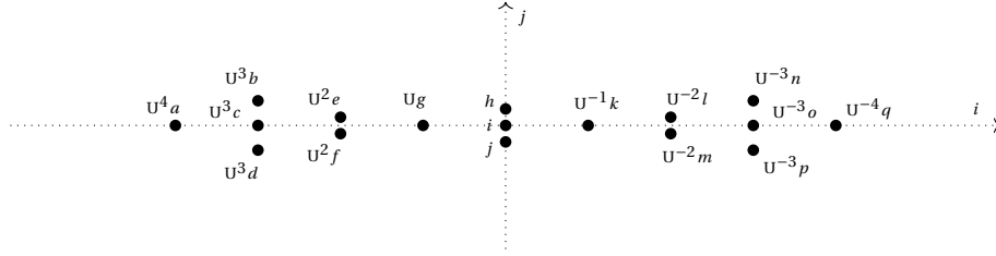
Figure 22: The arrangement of the generators of C\{j = 0\} . Note that U^{-3}n , U^{-3}o , and U^{-3}p all have homological grading 0.
