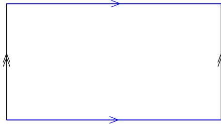
Figure 16: The torus can be represented as a rectangle with opposite sides identified.
