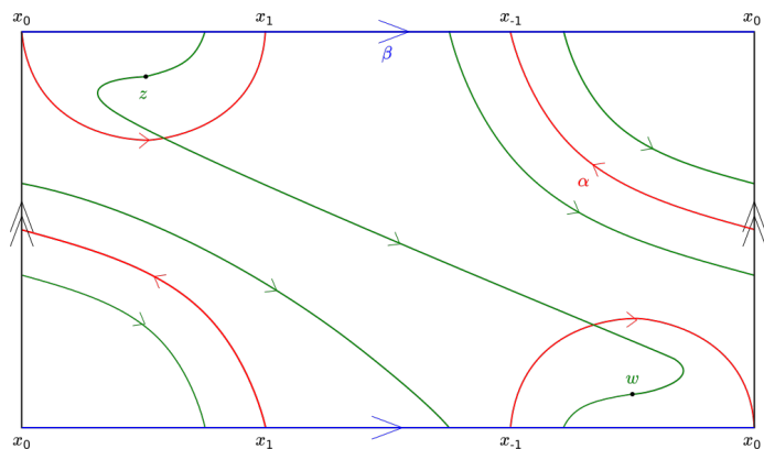
Figure 18: The Heegaard diagram for the right-handed trefoil knot, with the knot shown in green.
