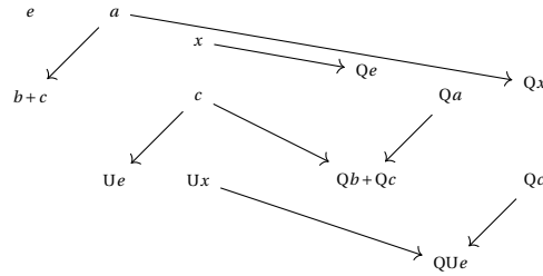
Figure 14: AI_0^- for the figure eight knot shown after applying a change of basis to the structure in Figure 13.
