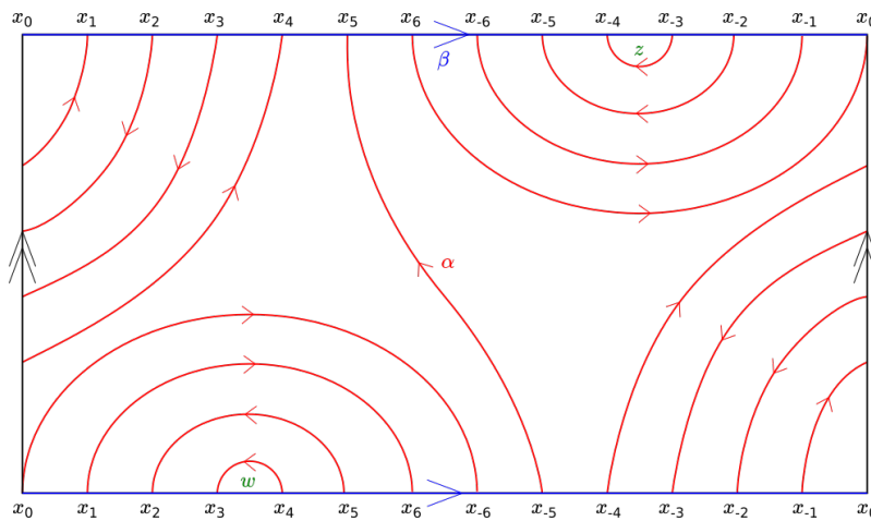
Figure 30: The (1,1) -diagram for 10_{161} has 13 intersection points, labelled by x_i for -6 \leq i \leq 6 , between the loops \alpha and \beta .
