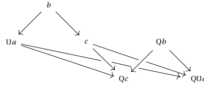
Figure 7: AI_0^- for the right-handed trefoil knot consists of all positive U -powers of the structure shown.
