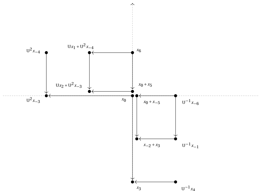
Figure 34: After the change of basis shown, CFK^\infty(10_{161}) consists of a staircase and two boxes.
