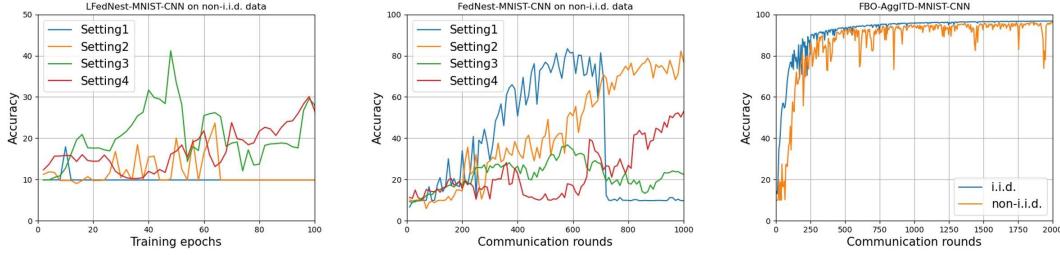
Figure 6. Performance of LFedNest, FedNest and FBO-AggITD on MNIST when the backbone is chosen as CNN and One-Round-Lower uses the SVRG-type method.
