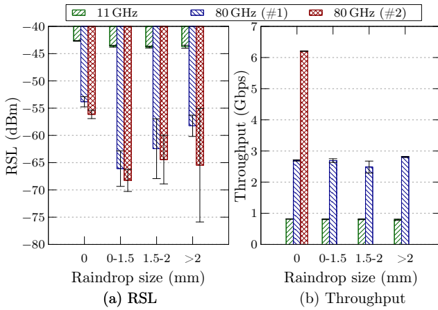
Fig. 7: Impact of raindrop size on AraHaul links (CI = 95%). available to the broad research community for further analysis. AraHaul is currently in beta test phase, and it is expected to be made available for public access in Fall 2023. Besides the example experiment shown in this article, AraHaul will enable a wide range of research investigations. For instance, once the AraOptical part of AraHaul becomes operational, it will further broaden the set of supported experiments within and across long-distance, high-capacity x-haul links at 11 GHz, 71–86 GHz, and 191.7–194.8 THz. AraHaul will also be able to support research investigations such as rigorous modeling of the dynamics, diversity, and weather sensitivity of long-distance, high-capacity wireless x-hauls, experimental study of wireless x-hauls in Open RAN architectures, as well as x-haul control and adaptation mechanisms to support application-specific Quality-of-Service (QoS) and Quality-of-Experience (QoE) requirements (e.g., those in real-time agricultural automation and XR-based rural education). Together, these research studies are expected to generate foundational insights and systems prototypes for next-generation x-haul solutions in rural broadband and advanced wireless in general.
