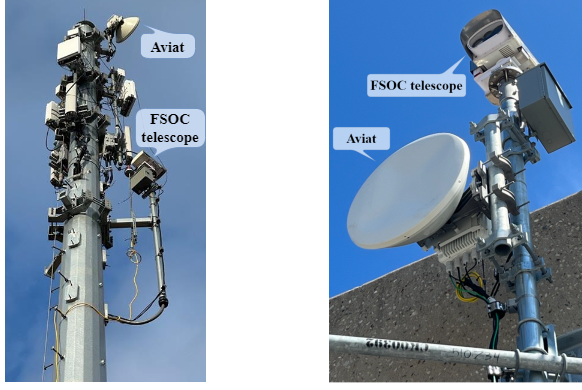
(a) Agronomy Farm site. (b) Wilson Hall site. Fig. 2: Aviat dish antennas and FSOC telescopes of AraHaul.
