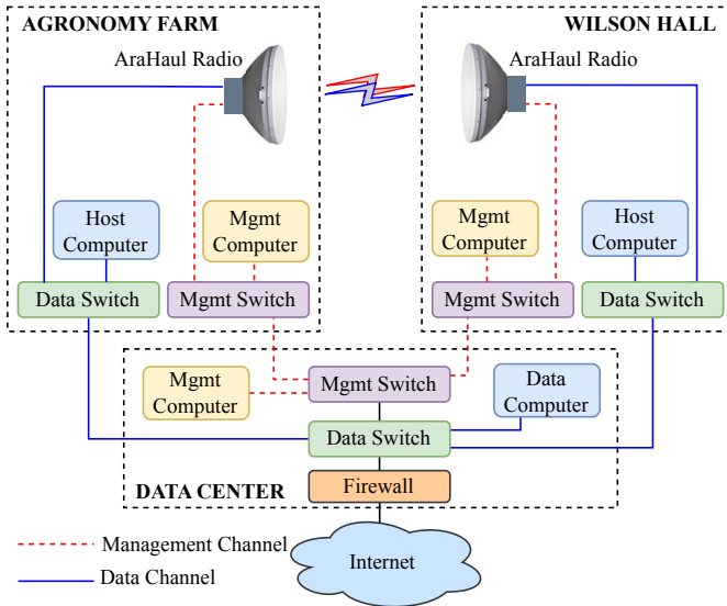
Fig. 3: AraHaul hardware and network architecture.
