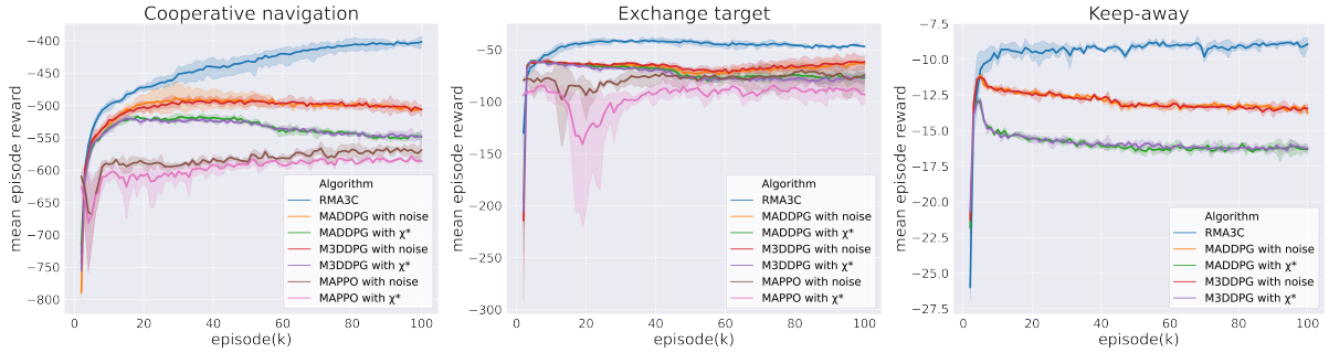
Figure 11: Our RMA3C algorithm compared with several baseline algorithms during the training process. The results showed that our RMA3C algorithm outperforms the baselines, achieving higher mean episode rewards and displaying greater robustness to state perturbations. The baselines were trained under either random state perturbations or a well-trained adversary policy \chi^* (adversaries that are trained for the maximum training episodes in RMA3C). Overall, our RMA3C algorithm achieved up to 58.46% higher mean episode rewards than the baselines.
