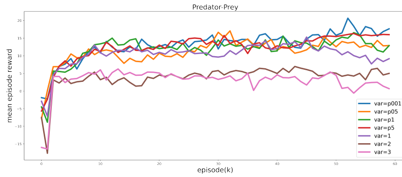
Figure 23: We train RMAAC policies using different values of variance in the scenario Predator-Prey. In general, the smaller the variance is used, the higher the mean episode rewards RMAAC can achieve.
