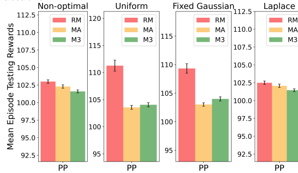
Figure 29: We test the performance of RMAAC policies under the attacks of different noise formats in the scenario Predator-Prey. RM denotes our robust MARL algorithm, i.e. RMAAC. MA denotes MADDPG, a MARL baseline algorithm. M3 denotes M3DDPG, a robust MARL baseline algorithm. Our RMAAC algorithm outperforms baseline algorithms in terms of mean episode testing rewards under all kinds of attacks.
