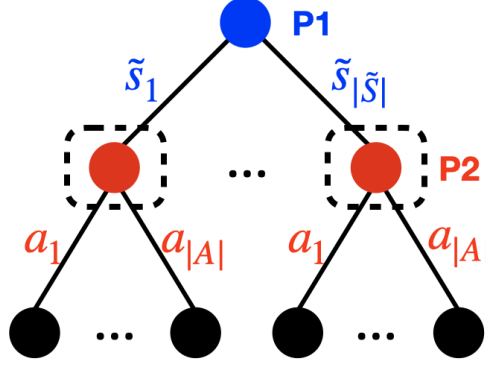
Figure 9: a team extensive-form game
