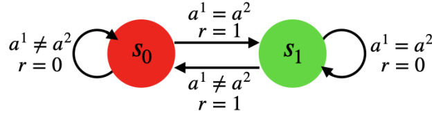
Figure 10: Two-player game: each player has two states and the same action set with size 2. Under state s_0 , two players get the same reward 1 when they choose the same action. At state s_1 , two players get the same reward 1 when they choose different actions. One state switches to another state only when two players get a reward, i.e. two players always stay in the current state until they get the reward.
