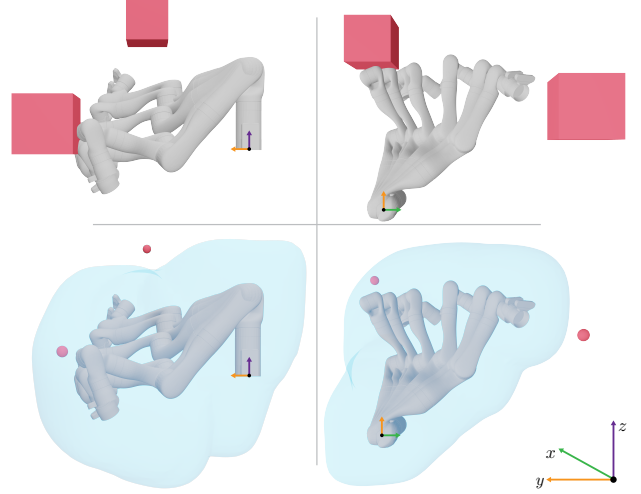
Fig. 1: RDF is a neural implicit safety representation that computes distances between the swept volume of a robotic arm and obstacles within a receding-horizon trajectory planning framework. The top panels show two different orthographic views of a single planning iteration with several intermediate poses of the robot arm in collision with one of the obstacles (red cubes). The bottom panels show orthographic views of the 3D reconstruction of RDFs signed distance field (transparent blue) with one of the obstacle centers (red spheres) interior to RDF’s zero-level set.
