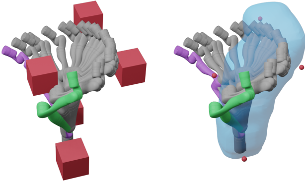
Fig. 4: Real-time receding-horizon trajectory planning with RDF in a cluttered environment. (Left) The arm safely moves from the start pose (purple) through intermediate configurations (grey) to reach the goal (green) while avoiding obstacles (red cubes). (Right) During the highlighted planning iteration all obstacle centers (red spheres) remain outside RDF's zero-level set (blue).
