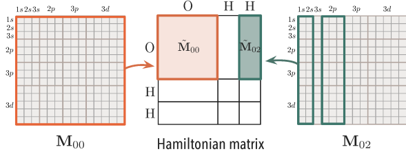
Figure 3. Construction of tensor matrix. The expansion module of our model outputs the intermediate block \mathbf{M} with full orbitals for each node pair. Then, pair block \tilde{\mathbf{M}} is selected from \mathbf{M} according to orbitals of corresponding atoms. Finally, the Hamiltonian matrix of a molecule is built by combining \tilde{\mathbf{M}} of all node pairs.
