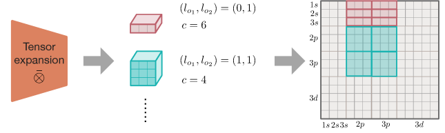
Figure 4. The relationship between the channel of equivariant matrix and the intermediate full orbital matrix. Here, c is the number of channel for equivariant matrices, and (l_{o1}, l_{o2}) is the rotation order of the equivariant matrix. Then, these equivariant matrices composed of the intermediate full orbital matrix for each node pair.
