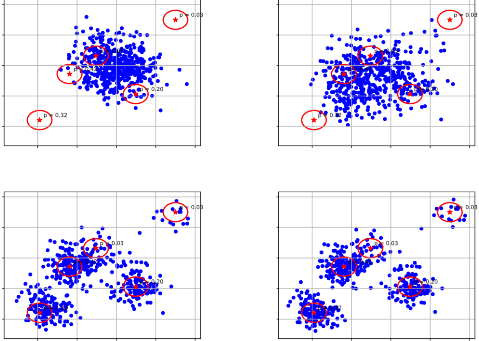
Figure 1: A realization of DPUM for a mixture of Gaussians.
