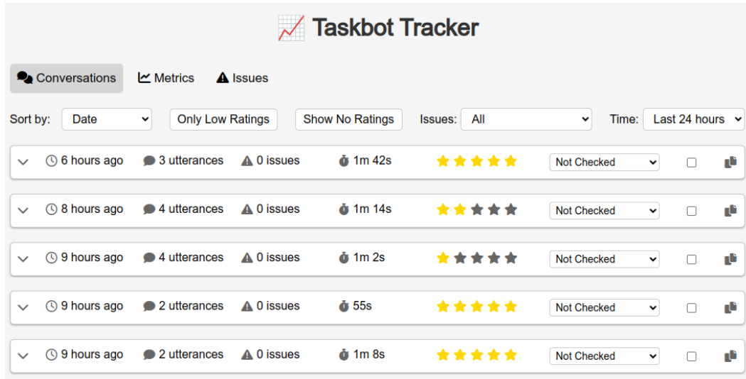
Figure 9: Taskbot Tracker: Tool for tracking user interactions and swiftly integrating feedback.
