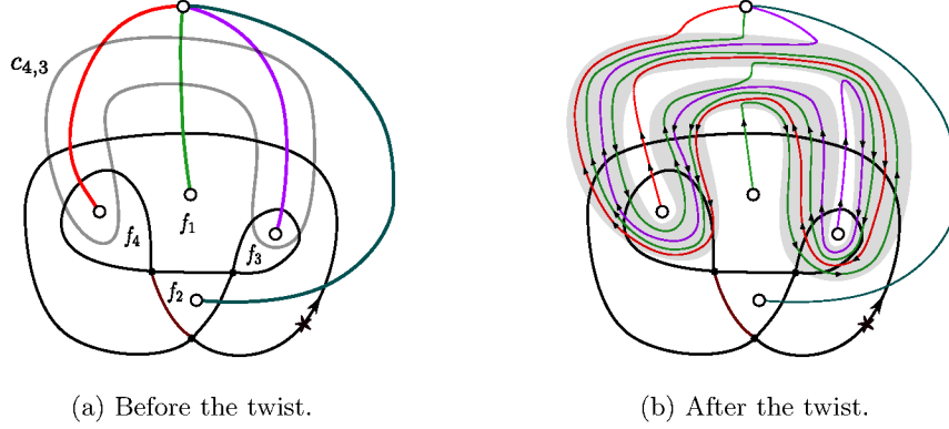
Fig. 15: (a) An example of the Dehn twist. The curve is shown in black. Starting from the star and following the indicated orientation, the Blank word is w = [23142\bar{3}4] . In the instance we have i = 4 and j = 3 ; the curve c_{4,3} is shown in gray. The word B is \mathbf{1} . (b) After twisting about an annulus formed by fattening c_{4,3} the new word is w' = [214\bar{1}33314\bar{1}141\bar{3}14\bar{1}314214\bar{1}3\bar{3}314\bar{1}41\bar{3}14\bar{1}314] .
