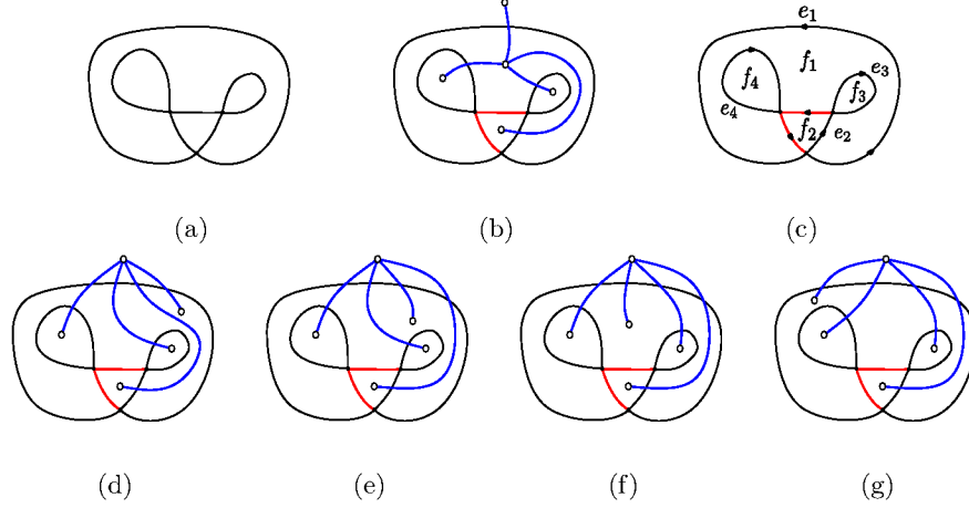
Fig. 13: (a) A curve \gamma . (b) A spanning tree in red and cotree in blue. (c) A labeling of the coedges and faces. We have four ways to break the cyclic face sequence for e_1 , represented using the cable system \Pi : (d) e_1 = \partial f_1 e_2 e_3 e_4 ; (e) e_1 = e_2 \partial f_1 e_3 e_4 ; (f) e_1 = e_2 e_3 \partial f_1 e_4 ; and (g) e_1 = e_2 e_3 e_4 \partial f_1 .
