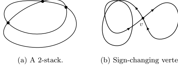
Fig. 16: (a) A k -stack where k = 2 . Smoothing at any of the three vertices gives a self-overlapping decomposition. (b) The vertex v is a sign-changing vertex.
