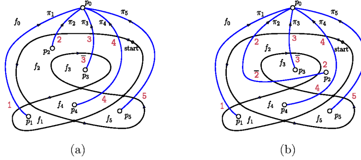
Fig. 11: (a) A curve with labeled faces and edges. A shortest path cable system \Pi_a is drawn in blue. From the indicated start position, the Blank Word is [\gamma]_B(\Pi_a) = [43254\bar{3}1] . (b) The same curve with a cable system \Pi_b that does not fulfill the shortest path assumption. The Blank word is [\gamma]_B(\Pi_b) = [43254\bar{2}321] .
