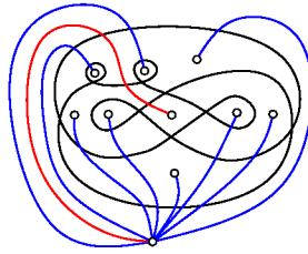
Fig. 10: An example of a cable system with a cable, in red, that cannot be managed.
