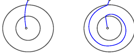
Fig. 14: An illustration of a Dehn twist.
