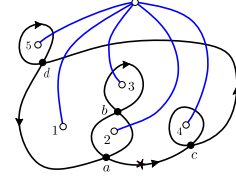
Fig. 8: A curve with combined word [c4c4231d5da2b3ba] .
