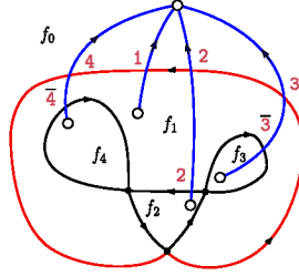
Fig. 12: As we traverse the red edge \gamma_r intersects 3 , 2 , then 1 —the cable corresponding to f_1 —then 4 . As we traverse the boundary of f_1 we traverse the red edge, followed by 4 and 23 . This choice of cable system \Pi corresponds to cycle flattening at f_1 as 2332144 by writing f_1 = \bar{e}_2 e_3 e_1 e_4 , or equivalently, 2332144 = \bar{e}_2 e_3 e_1 e_4 . The Blank subword on \gamma_r , with respect to the cycle flattening, is e_1 = \bar{3}2 \cdot \bar{2}332144 \cdot \bar{4} = 3214 , as expected.
