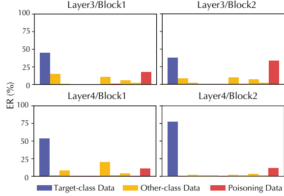
Figure 5: Entanglement ratios of the truncated encoder f_{l,k} .
