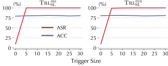
Figure 14: Attack performance of \text{TR}_{\text{SL}}^{\text{uni}} and \text{TR}_{\text{SL}}^{\text{dyn}} with respect to trigger strength (image patch size).
