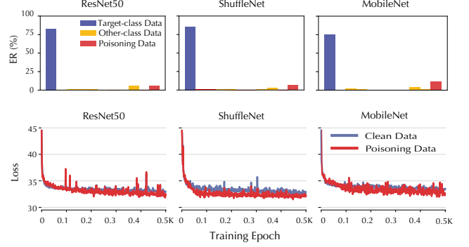
Figure 11: Learning dynamics and entanglement ratio under different backbone architectures.
