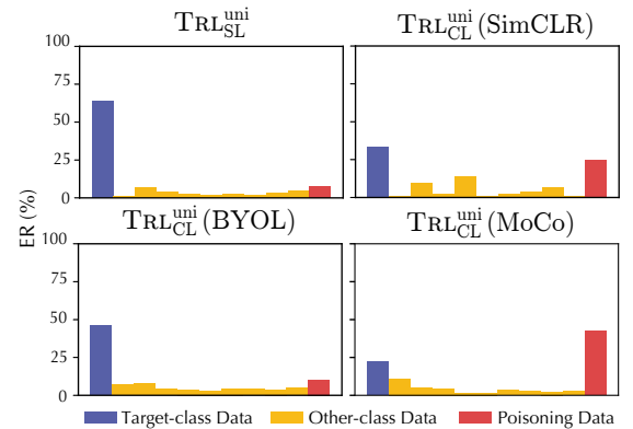
Figure 13: Entanglement ratios of \text{TRL}_{\text{SL/CL}}^{\text{uni}} on CIFAR10.
