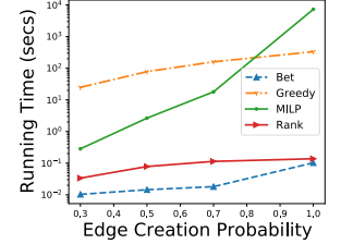
Figure 9: Running time (mean) v.s. Edge Creation Prob. in ER networks.
