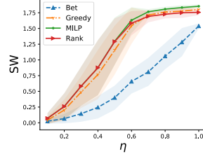
Figure 3: SW v.s. \eta of BA networks, B = 32 over total |\mathcal{E}^{in}| = 87
