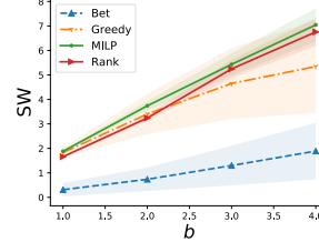
Figure 4: SW v.s. budget factor in Complete networks, \eta = 0.5
