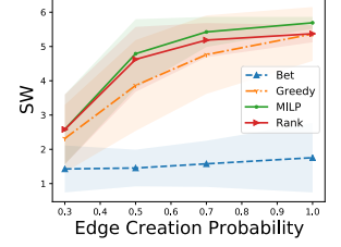
Figure 5: SW v.s. Edge Creation Probability in ER networks. \eta = 0.5 , b = 3.0
