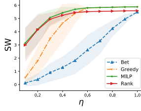
Figure 2: SW v.s. \eta of Complete networks, B = 96 over total |\mathcal{E}^{in}| = 1024
