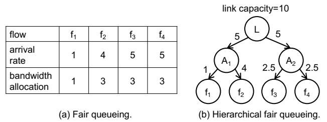
Figure 2: Fair queueing and hierarchical fair queueing.
