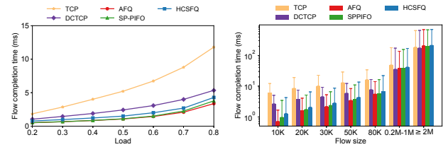
Figure 15: Simulation result under the web search workload.
