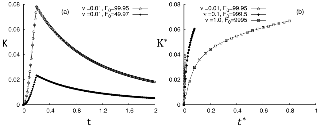
FIG. 9. (a) Kinetic energy per unit mass ( K in \text{cm}^2/\text{s}^2 ) vs time in seconds for the cases shown in the graph for T1 and T2. (b) Nondimensional velocity K^* = \sqrt{\frac{K}{F_0 l_f}} vs t^* for three cases in T1.
