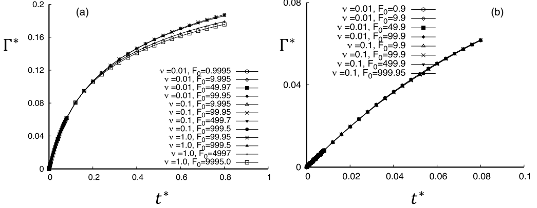
FIG. 7. Nondimensional circulation, \Gamma^* = \text{Re}_f \text{Re}_f^{-2} , vs nondimensional time, t^* = \frac{t\nu}{l_f^2} , in T1. (a) All cases, (b) cases \nu = 10^{-2} \text{ cm}^2/\text{s} and 10^{-1} \text{ cm}^2/\text{s} for all F_0 values.
