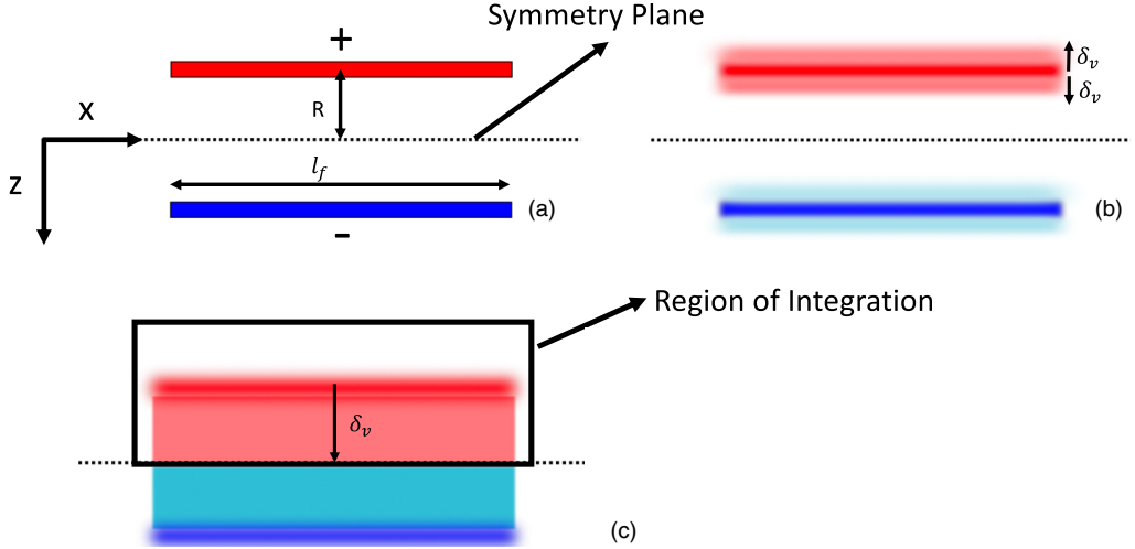
FIG. 11. Schematic representation of the lateral diffusion of vertical vorticity in T1. (a) Representation of the positive (red) and negative (blue) vertical vorticity layers immediately after the force acts on the fluid. This corresponds to the vorticity field shown in Fig. 4(a). (b) The vorticity is shown at a later time where it is seen to diffuse in the positive and negative z -direction from the red region. The viscous layer thickness is \delta_v . (c) The vorticity is shown at a time t \sim R^2/4\nu . Here the vorticity is shown diffusing from the red layer in the positive z -direction. The viscous layer thickness has reached the symmetry plane such that its thickness is approximately equal to the force radius, \delta_v \sim R . The circulation is determined by integrating the vertical vorticity over the region of integration shown.
