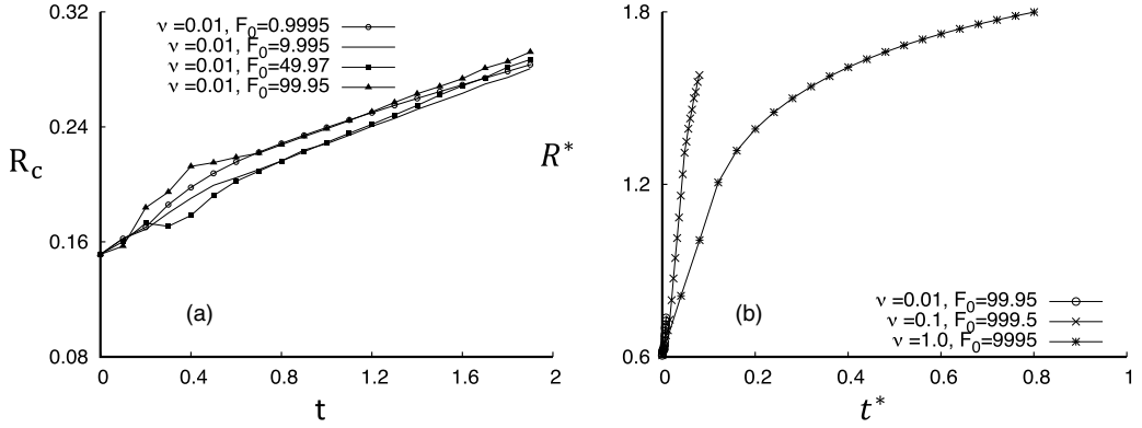
FIG. 8. (a) Equivalent core radius R_c (in cm) vs time in seconds for the cases shown in the graph. T1 and T2 are shown. The force turns off at t = 0.2 s. (b) Nondimensional equivalent core radius ( R^* = \frac{R_c}{R} ) vs t^* for all cases shown in the graph for T1.
