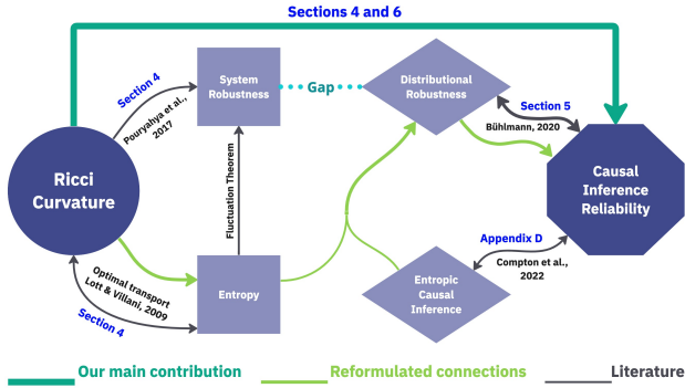
Figure 1: Visual summary of our theoretical contributions connecting the network geometry, via Ricci curvature, and causal inference. Our theory and methodological contributions are based in putting together novel results (e.g., filling the gap between different types of robustness), reformulating some of the existing links between relevant concepts in the literature, and connecting between different areas of machine learning. Arrow annotations mark the sections where the corresponding link is discussed and/or the most relevant related literature.
