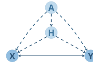
Figure 3: Causal graph for the anchor regression model. A , H , X , and Y denote the anchor, hidden confounders, covariates, and outcome.
