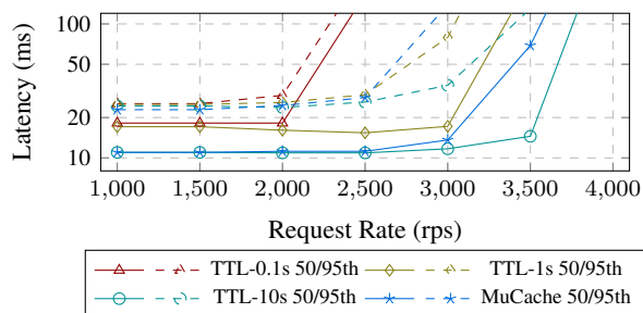
FIGURE 11—HotelRes: Latency and throughput of MuCache compared with various TTL.
