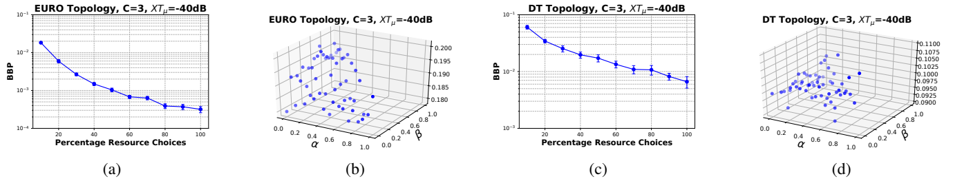
Figure 1: Variation in BBP for limited percentage of RCs for XT_{\mu} = -40\text{dB} and for different values of \alpha and \beta for EURO topology in Fig.1a and Fig.1b, respectively, and for DT topology in Fig.1c and Fig.1d, respectively.
