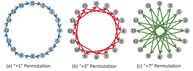
Figure 7: Ring-AllReduce permutations.
