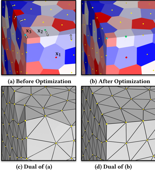
Fig. 3. The RVD after optimizing the positions by minimizing our objective function, points near the features are naturally drawn toward the nearby points/lines. In this figure, x_1 (red) controls a planar region and remains static, x_2 (green) dominates an area across the feature line and is shifted to the feature line, and x_3 (blue) governs a corner point and is relocated to the corner.
