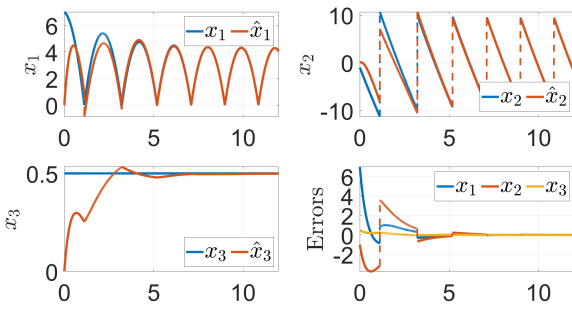
Fig. 1. State and parameter estimation in a bouncing ball.
